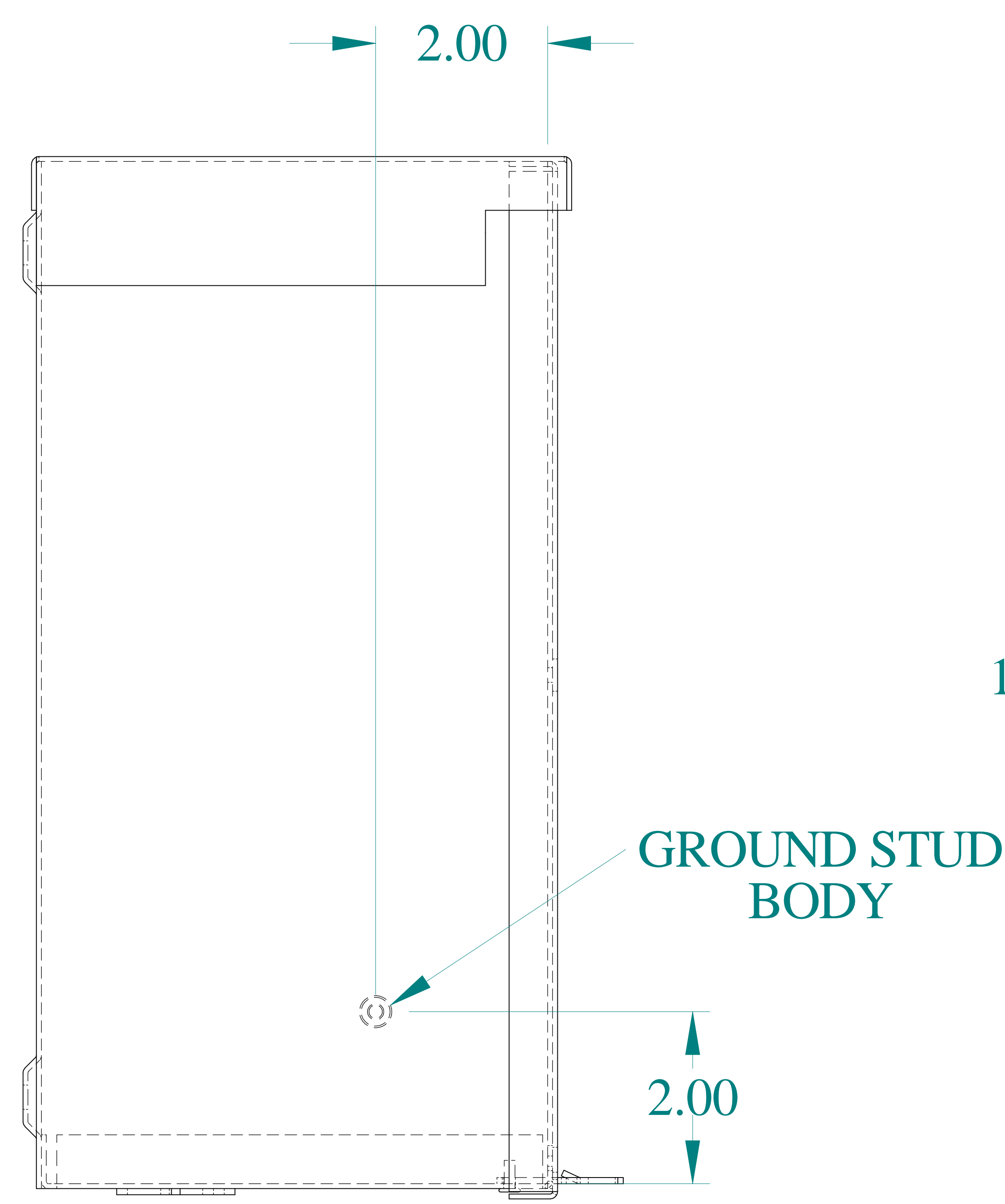
SIDE VIEW
