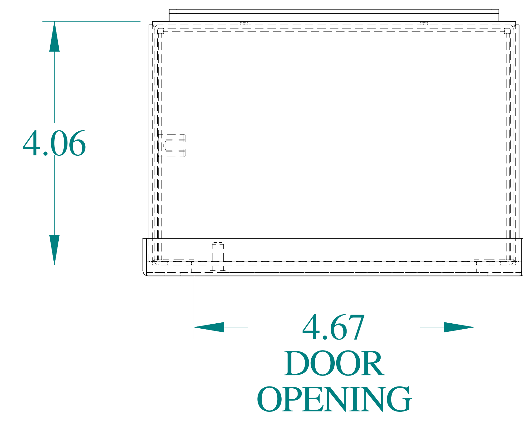
TOP VIEW
