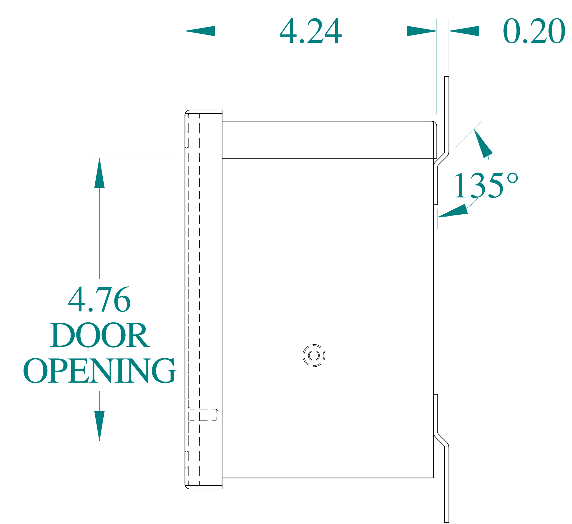
SIDE VIEW
