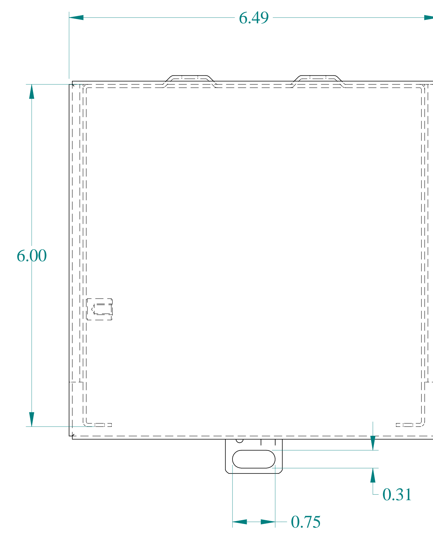
TOP VIEW
