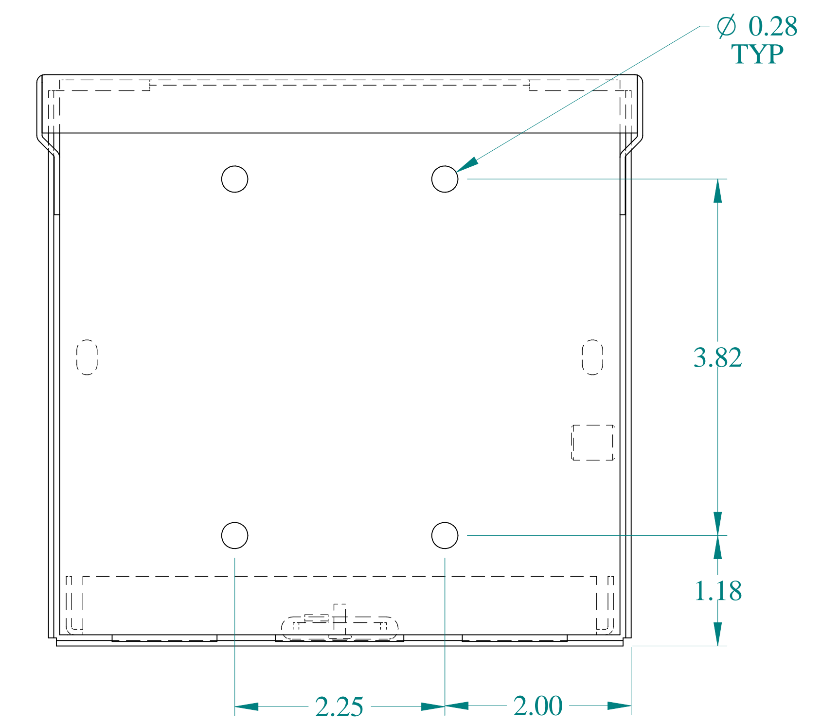
BACK VIEW
