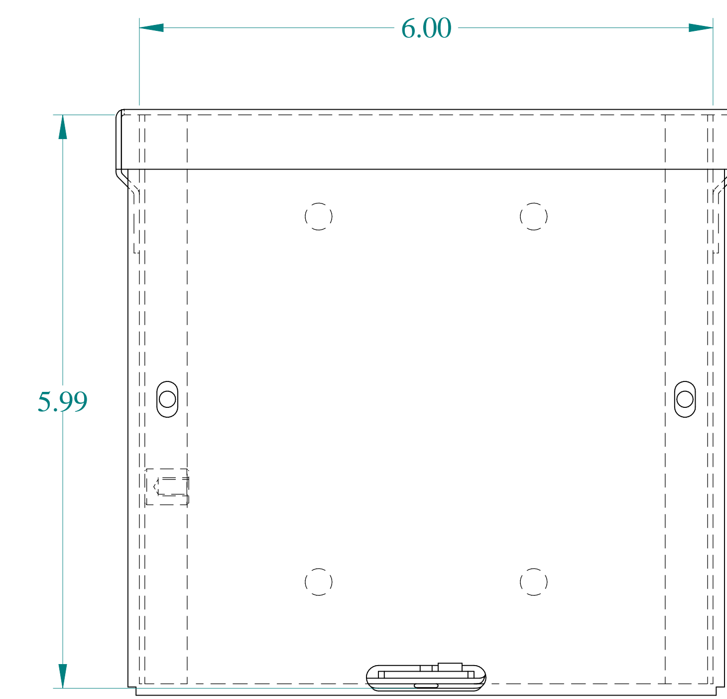
FRONT VIEW
