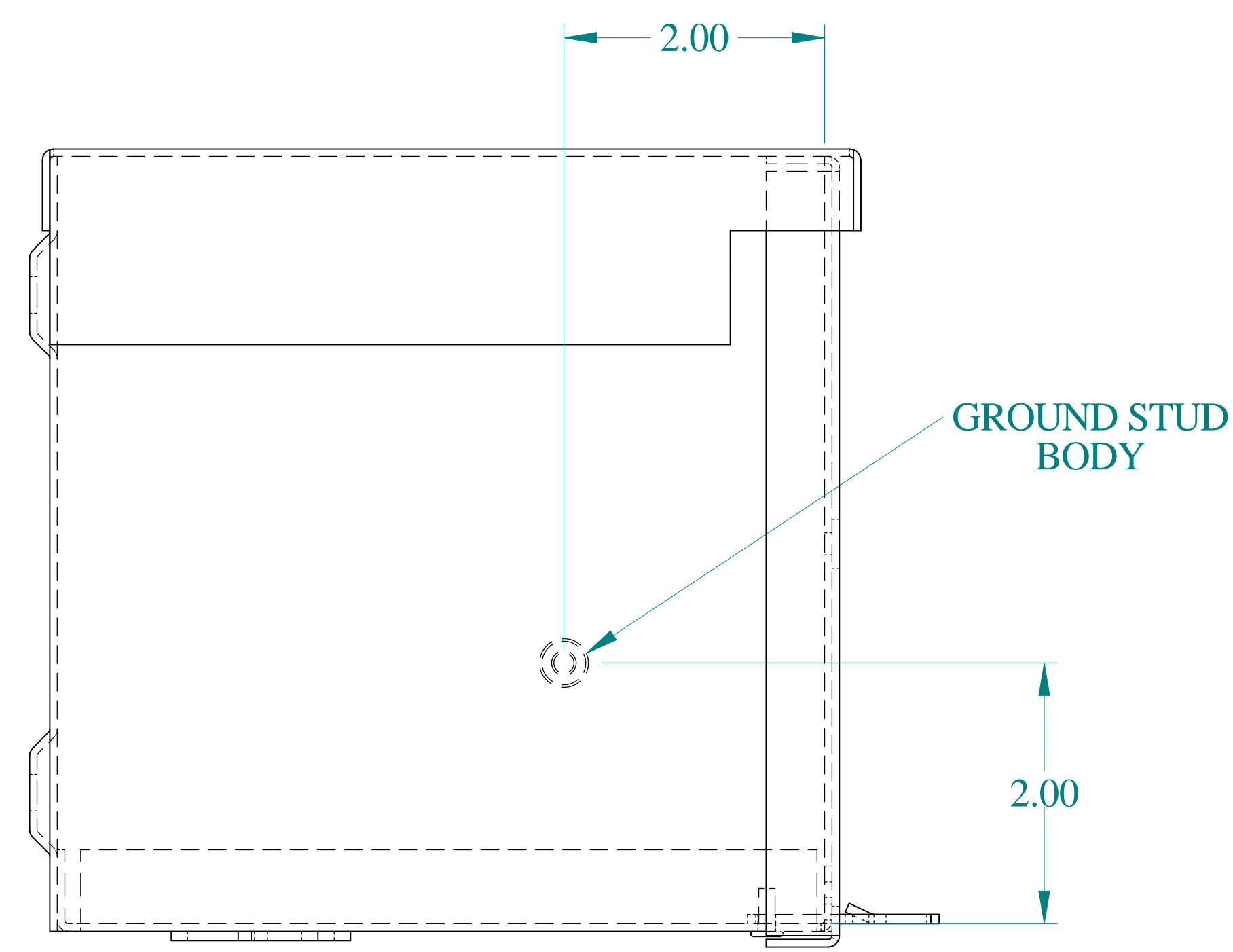
SIDE VIEW
