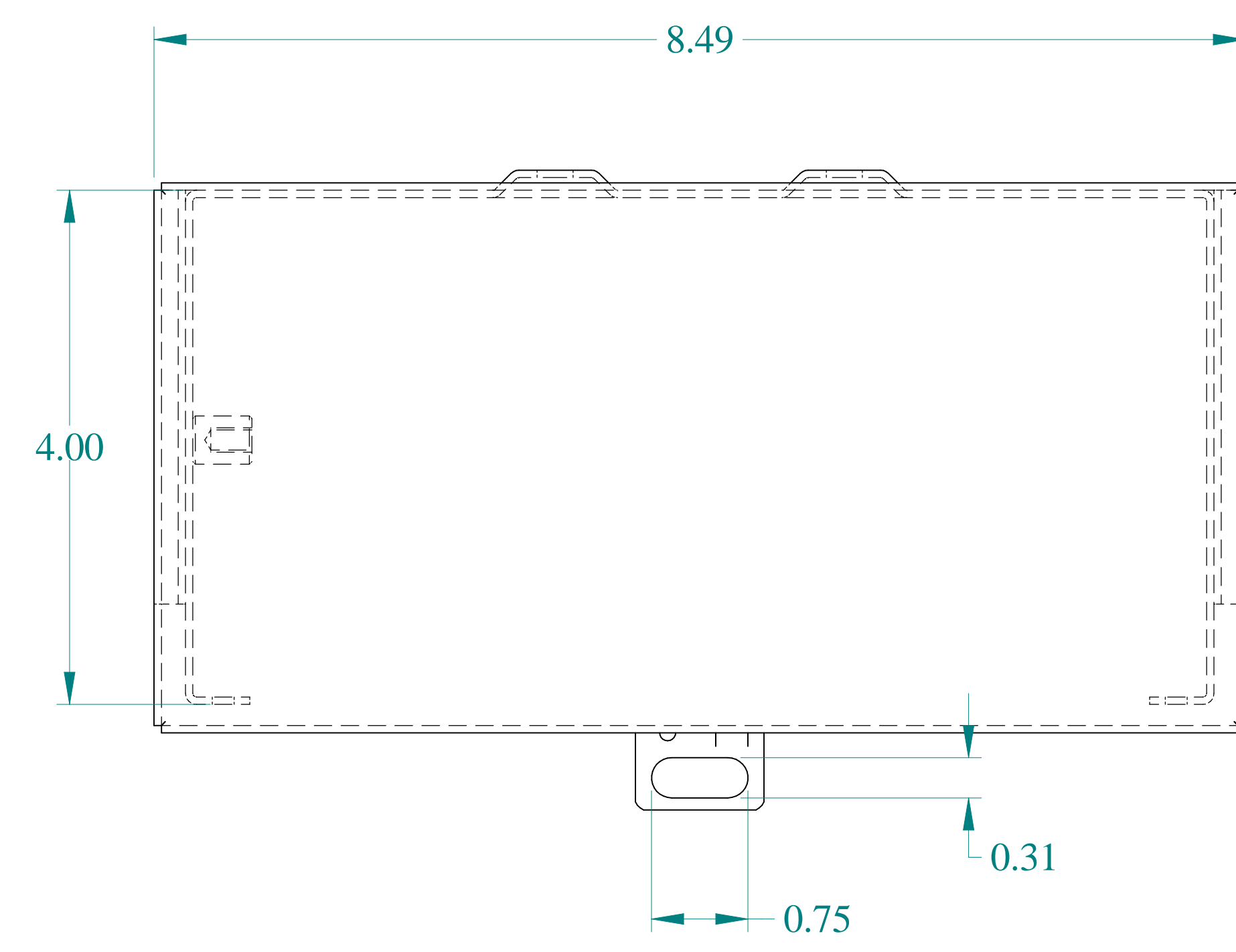
TOP VIEW
