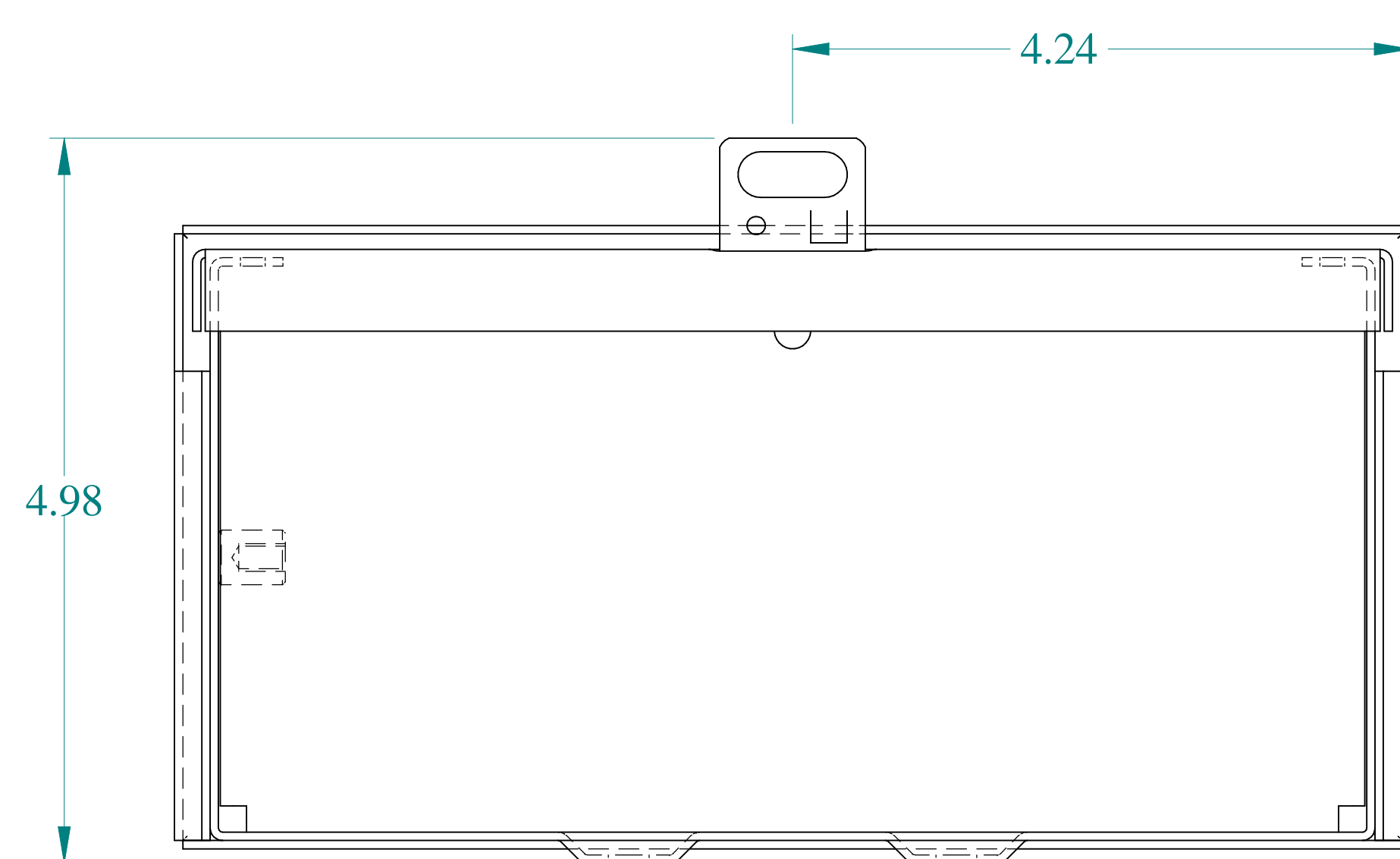
BOTTOM VIEW
