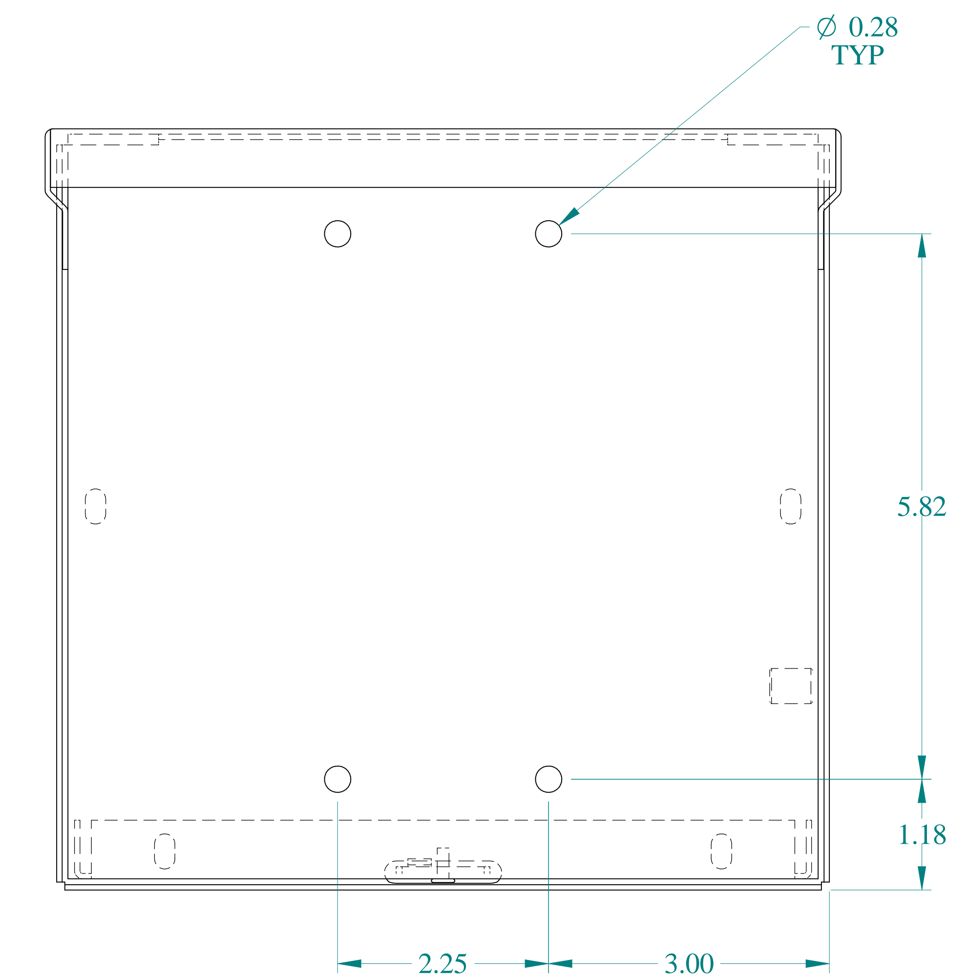
BACK VIEW
