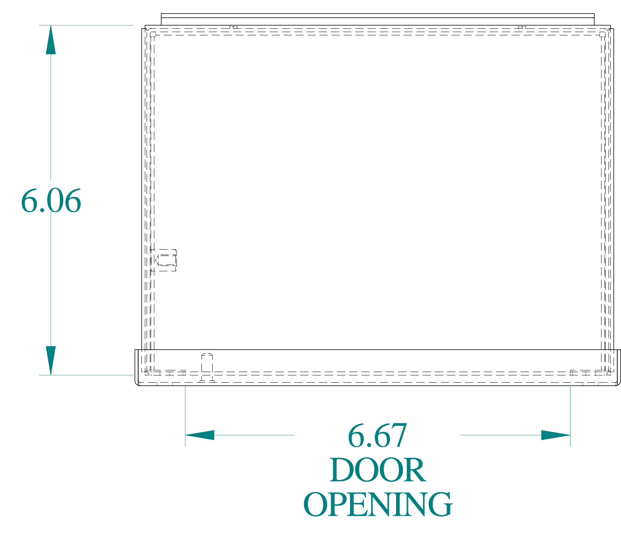
TOP VIEW
