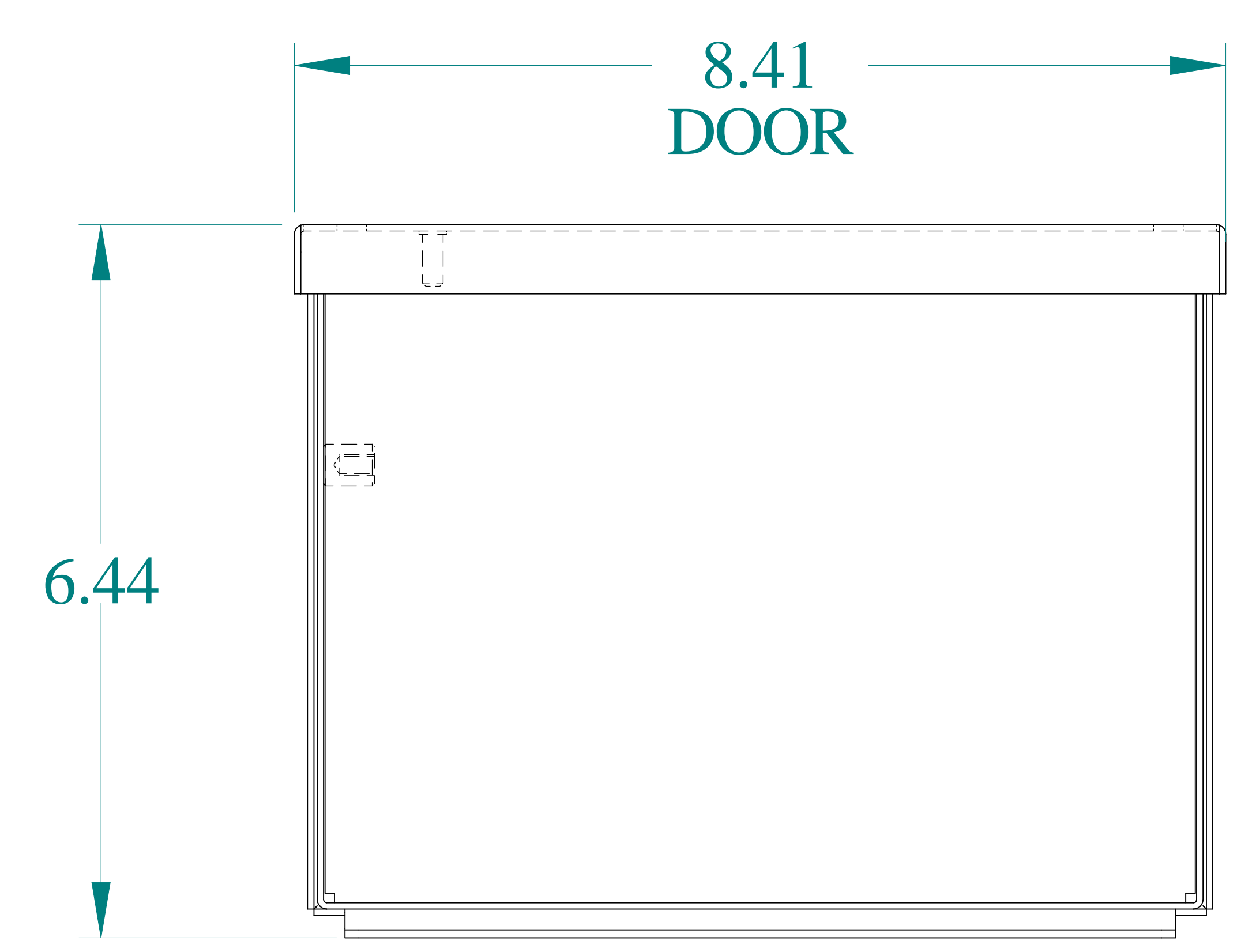
BOTTOM VIEW
