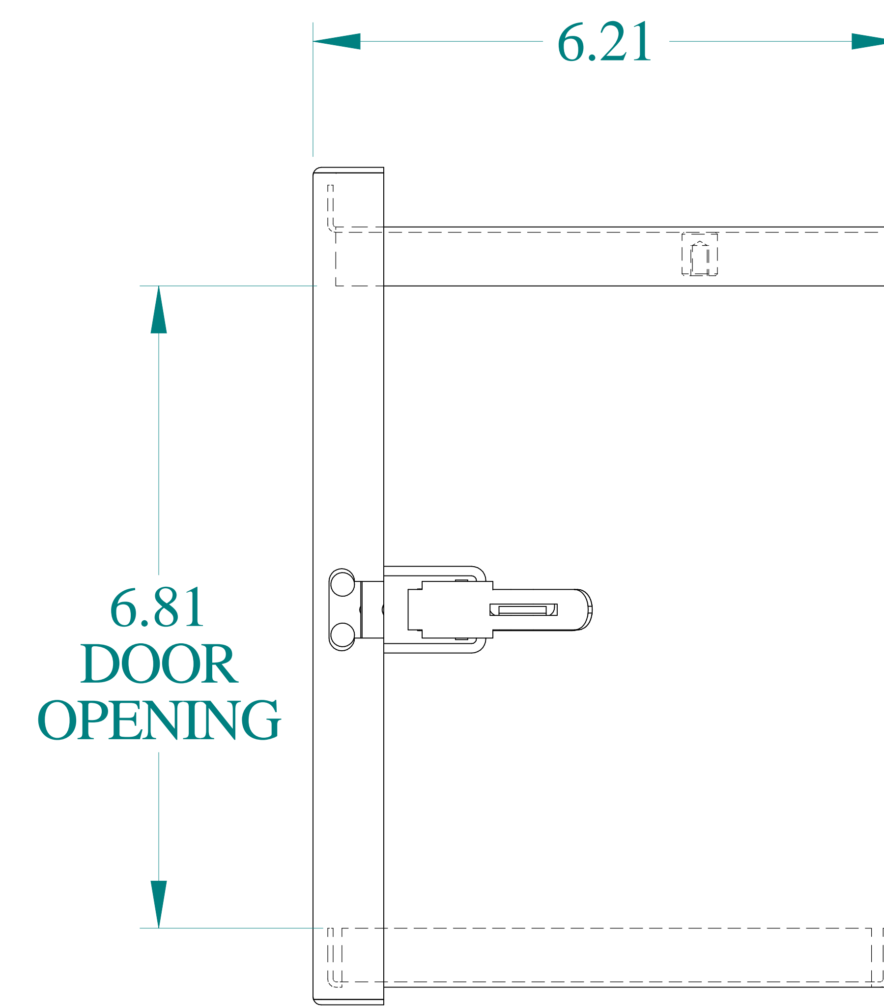
SIDE VIEW
