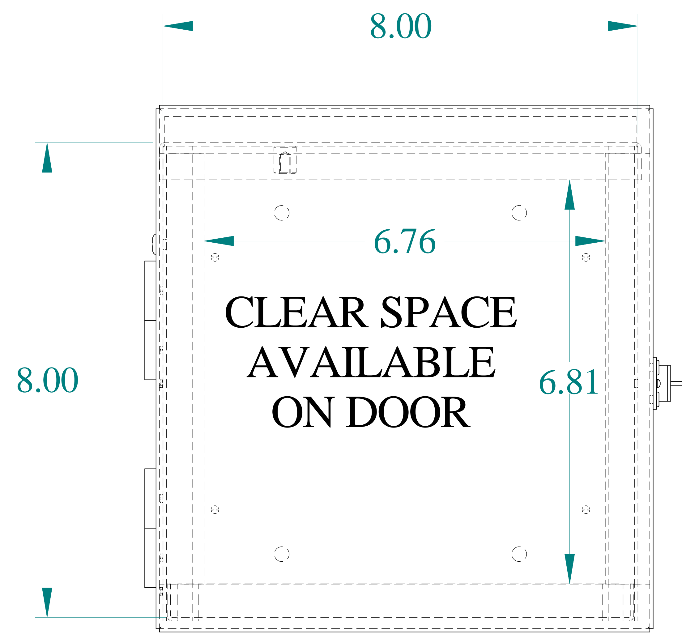
FRONT VIEW
