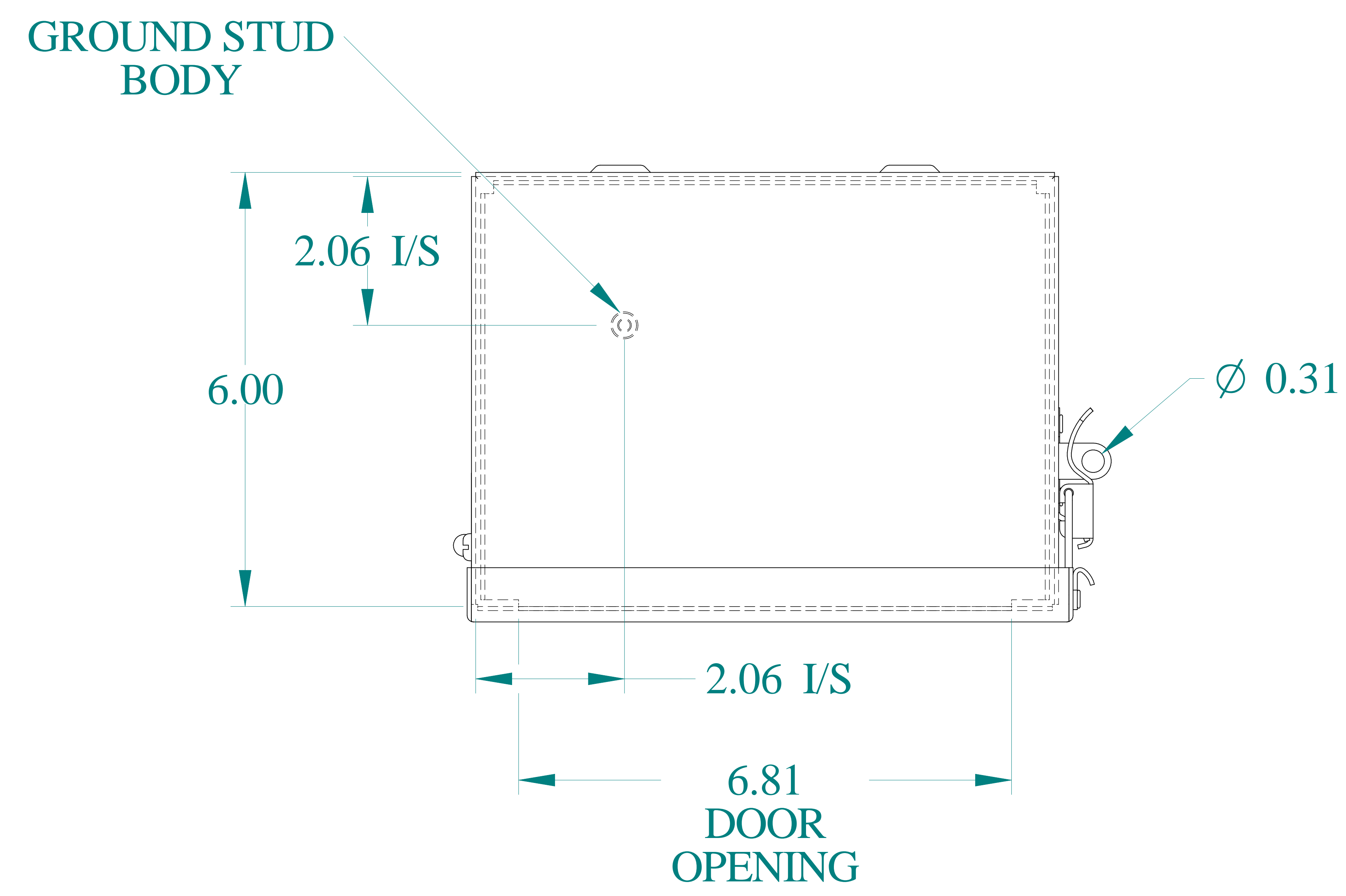
TOP VIEW
