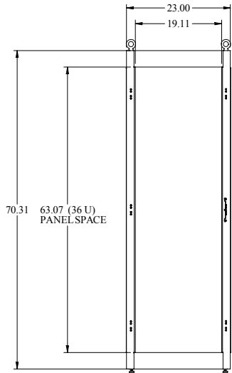
FRONT VIEW (DOORS REMOVED)
