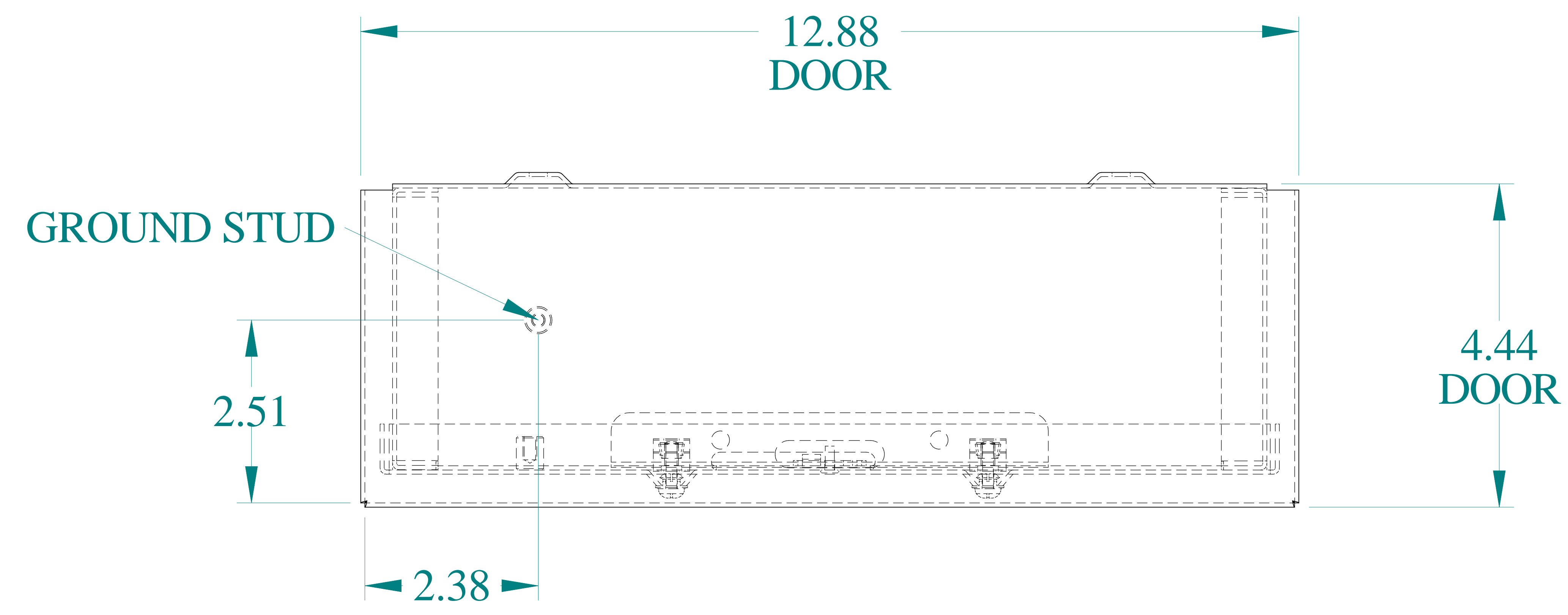
TOP VIEW
