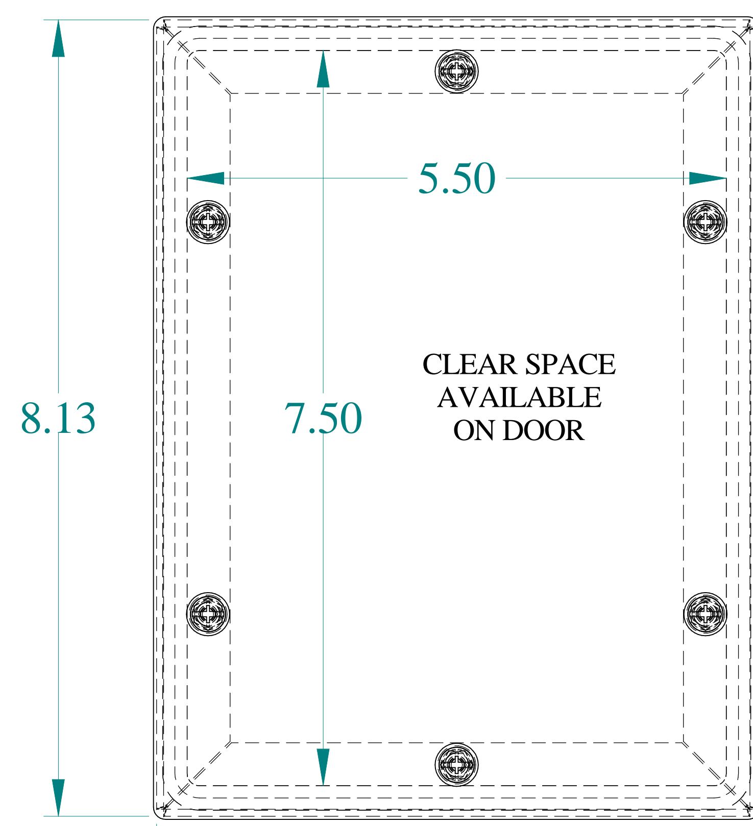
FRONT VIEW
