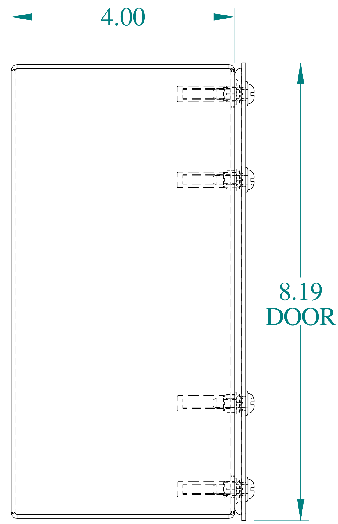
SIDE VIEW
