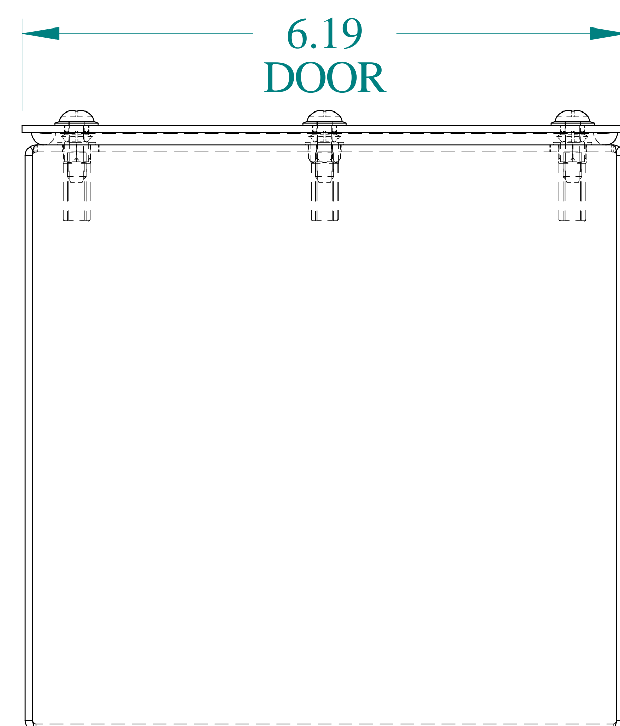
BOTTOM VIEW
