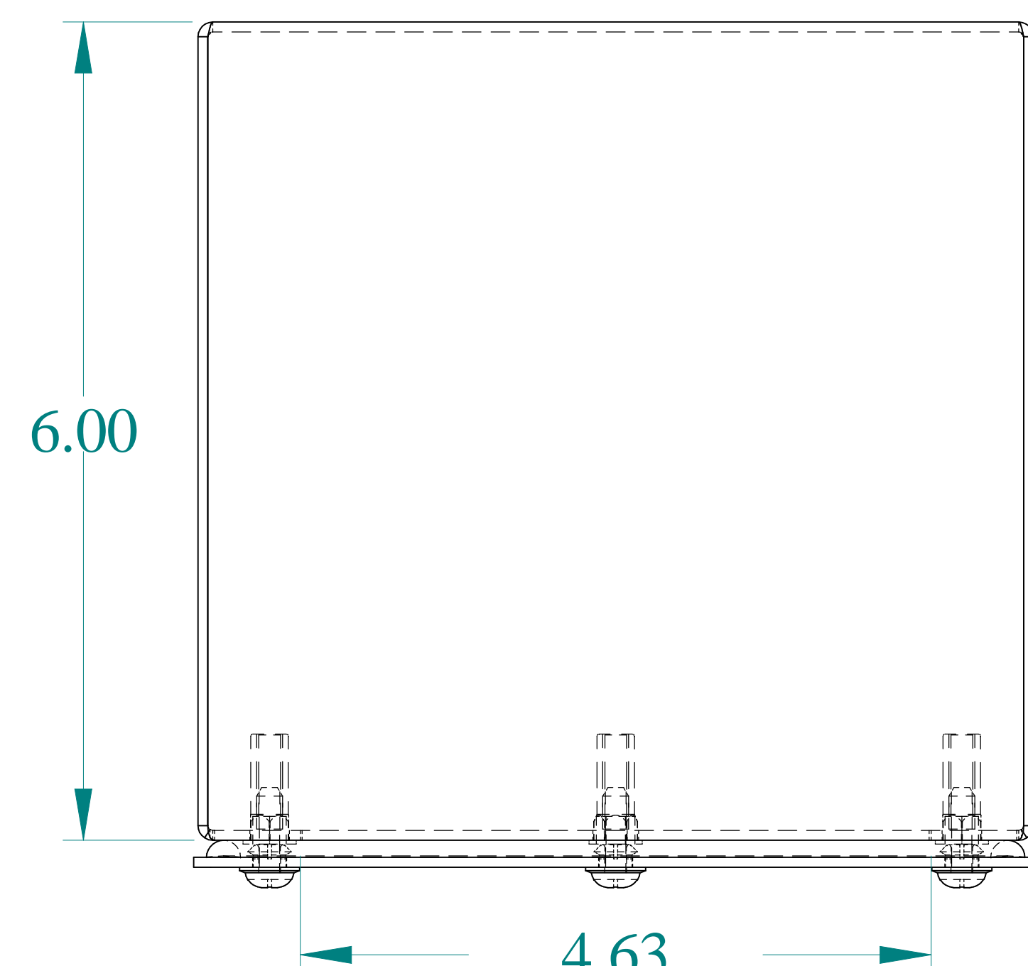
TOP VIEW
