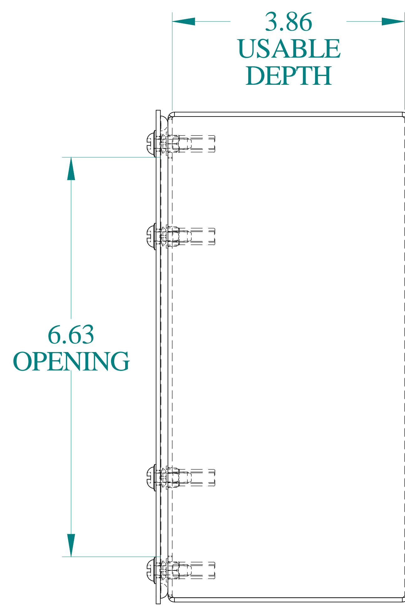
SIDE VIEW
