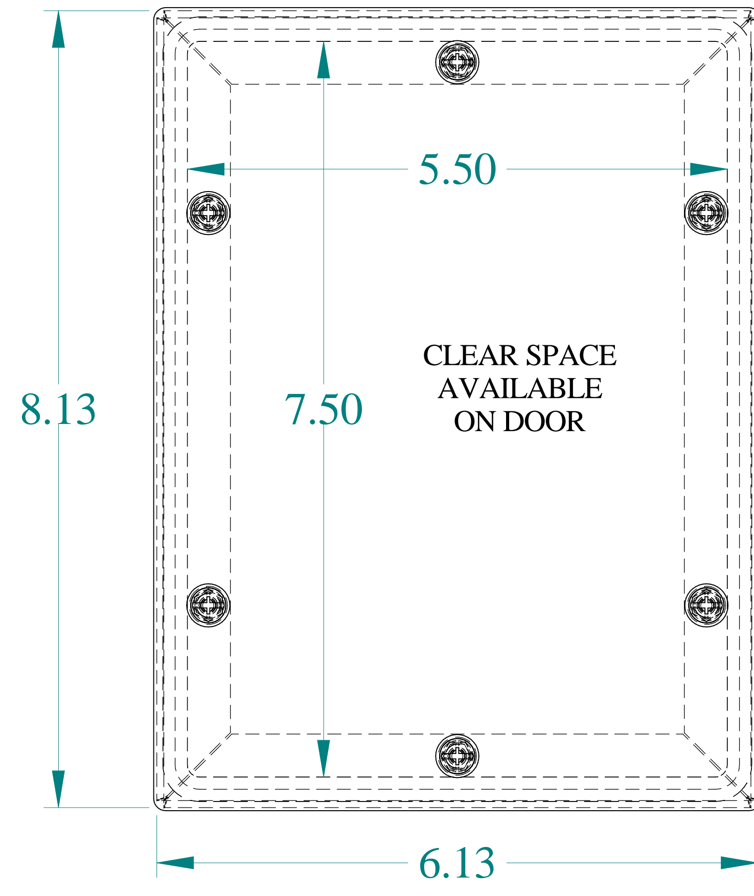
FRONT VIEW
