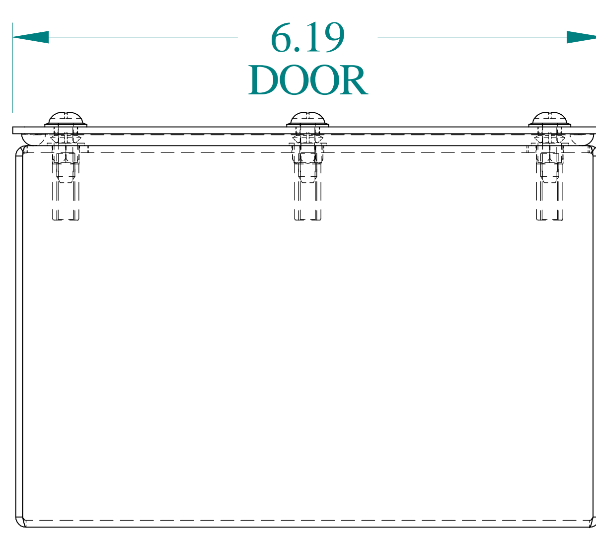
BOTTOM VIEW
