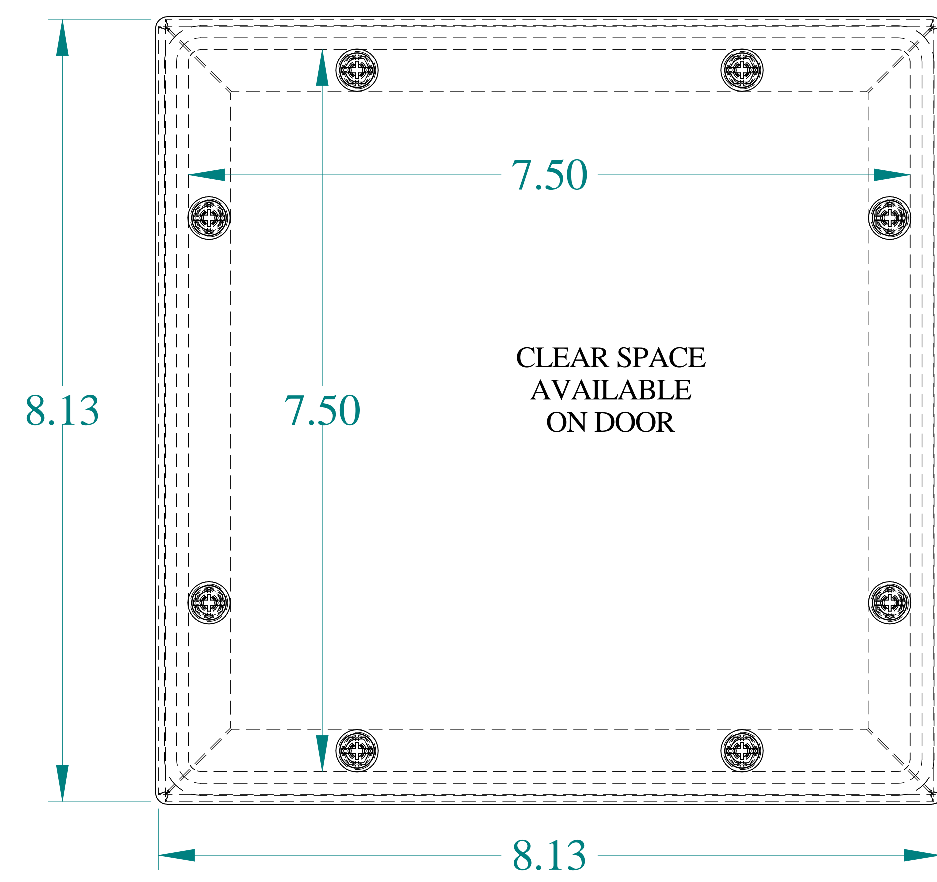
FRONT VIEW
