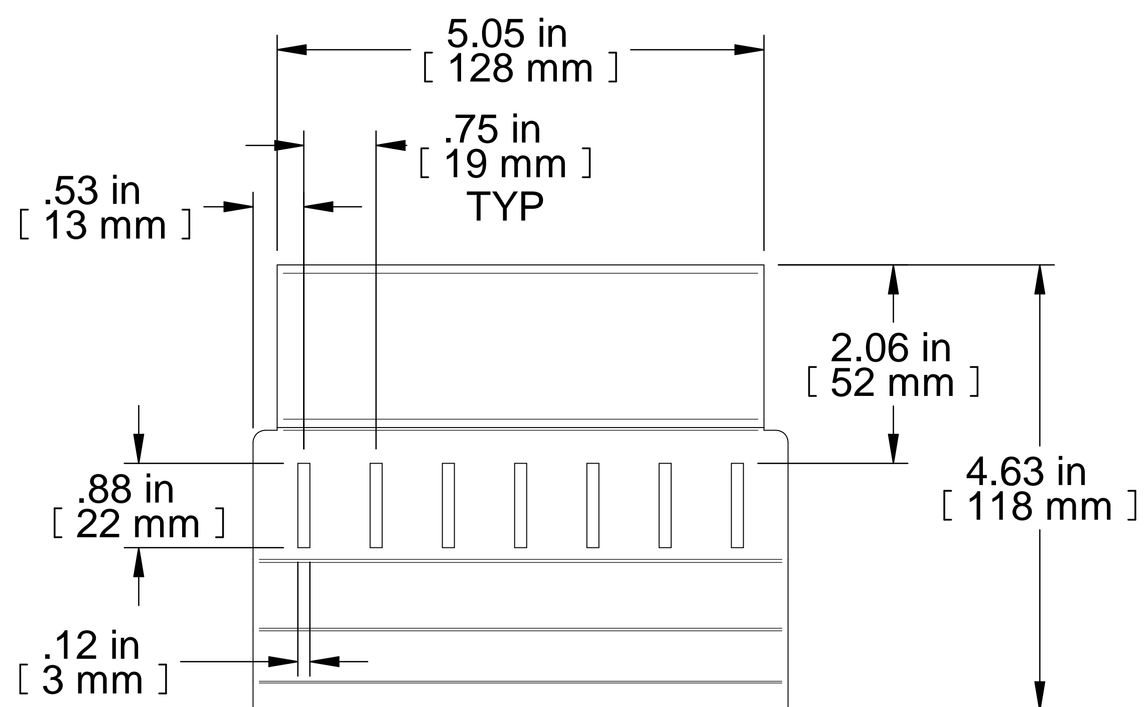
TOP VIEW
