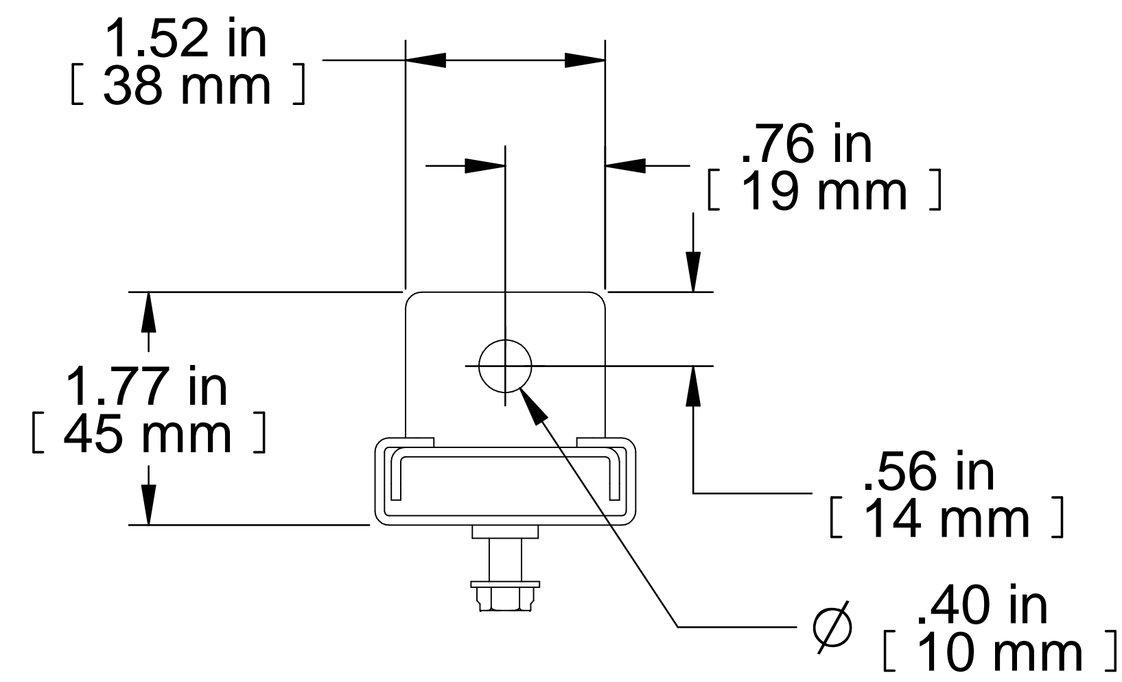
TOP VIEW
