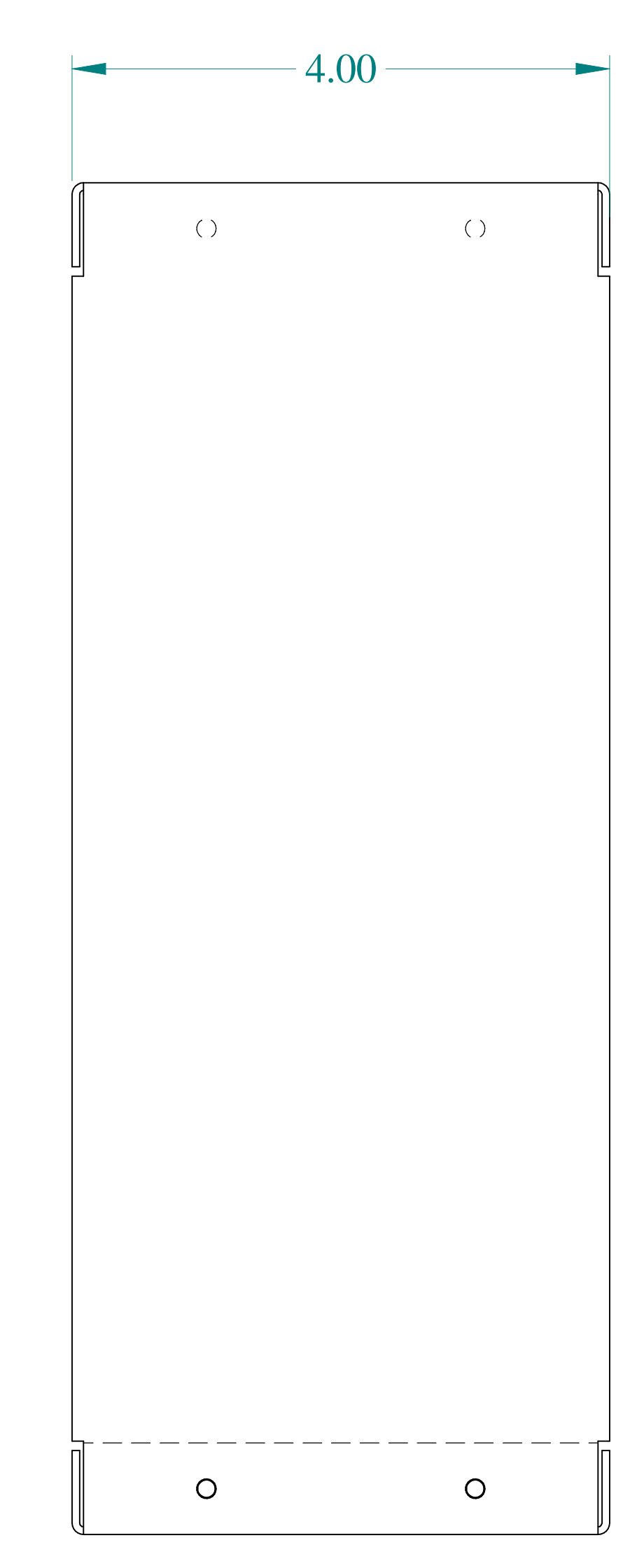
SIDE VIEW
