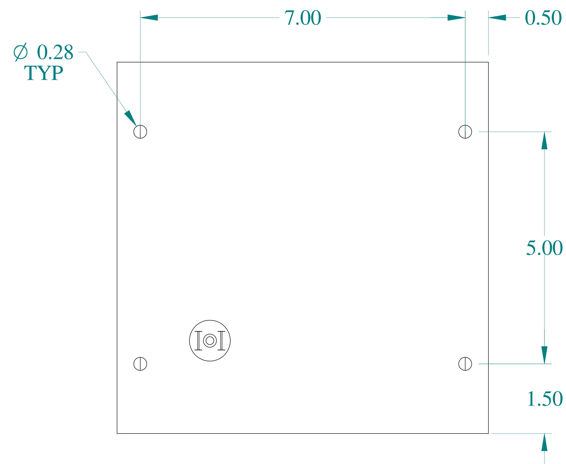
BOTTOM VIEW
