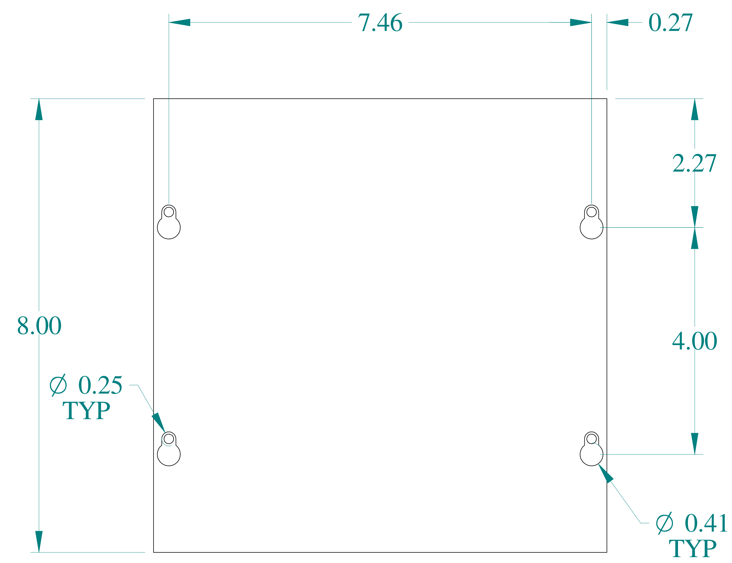
TOP VIEW
