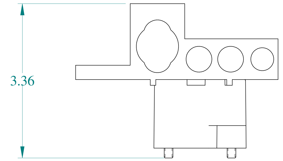
BACK VIEW
