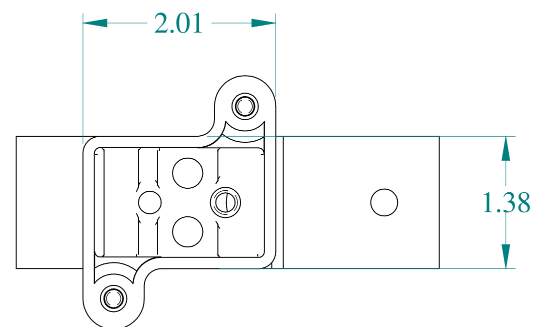
BOTTOM VIEW
