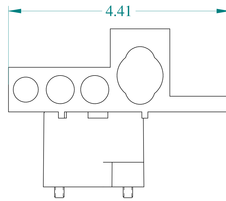
FRONT VIEW
