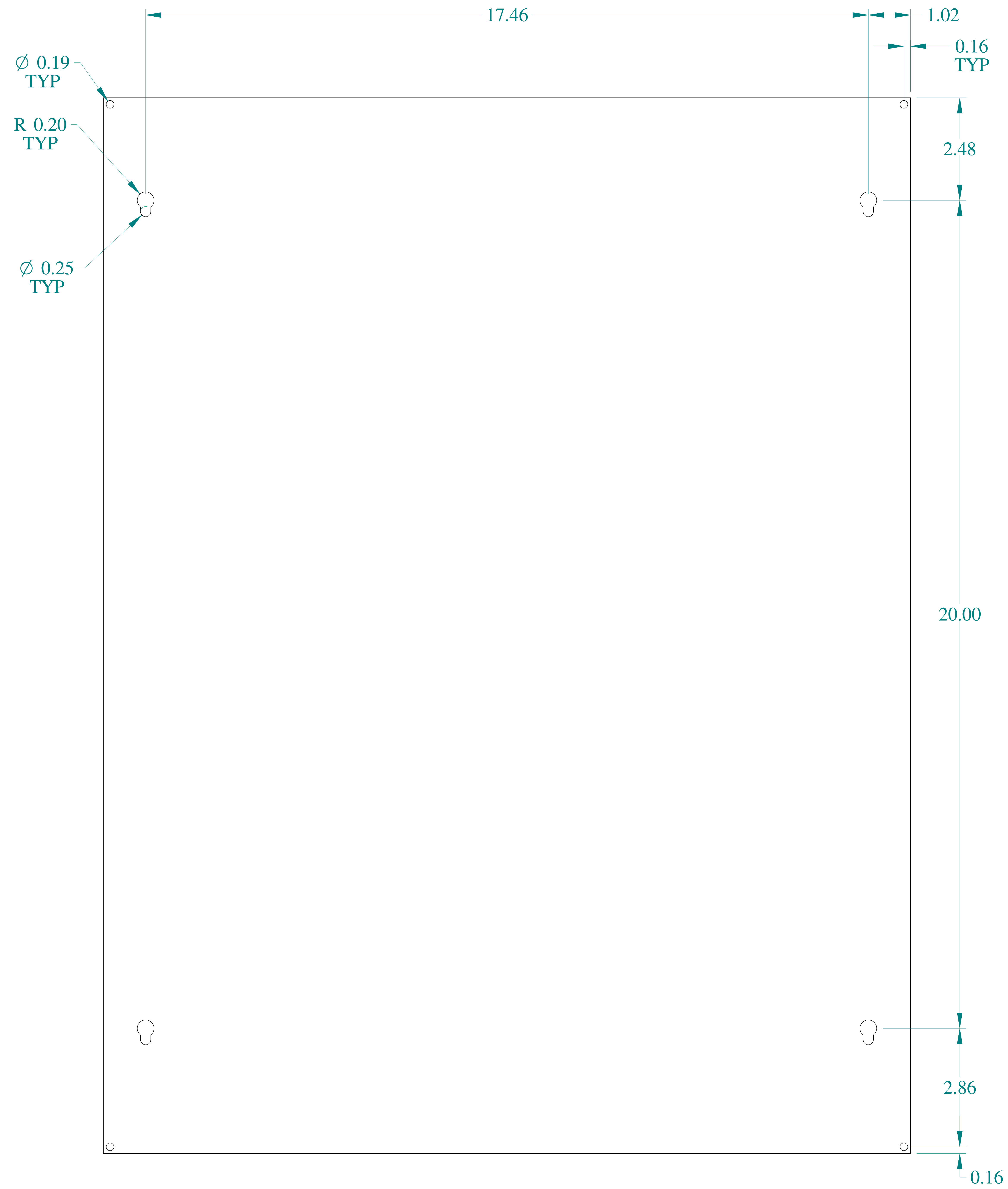
FRONT VIEW
