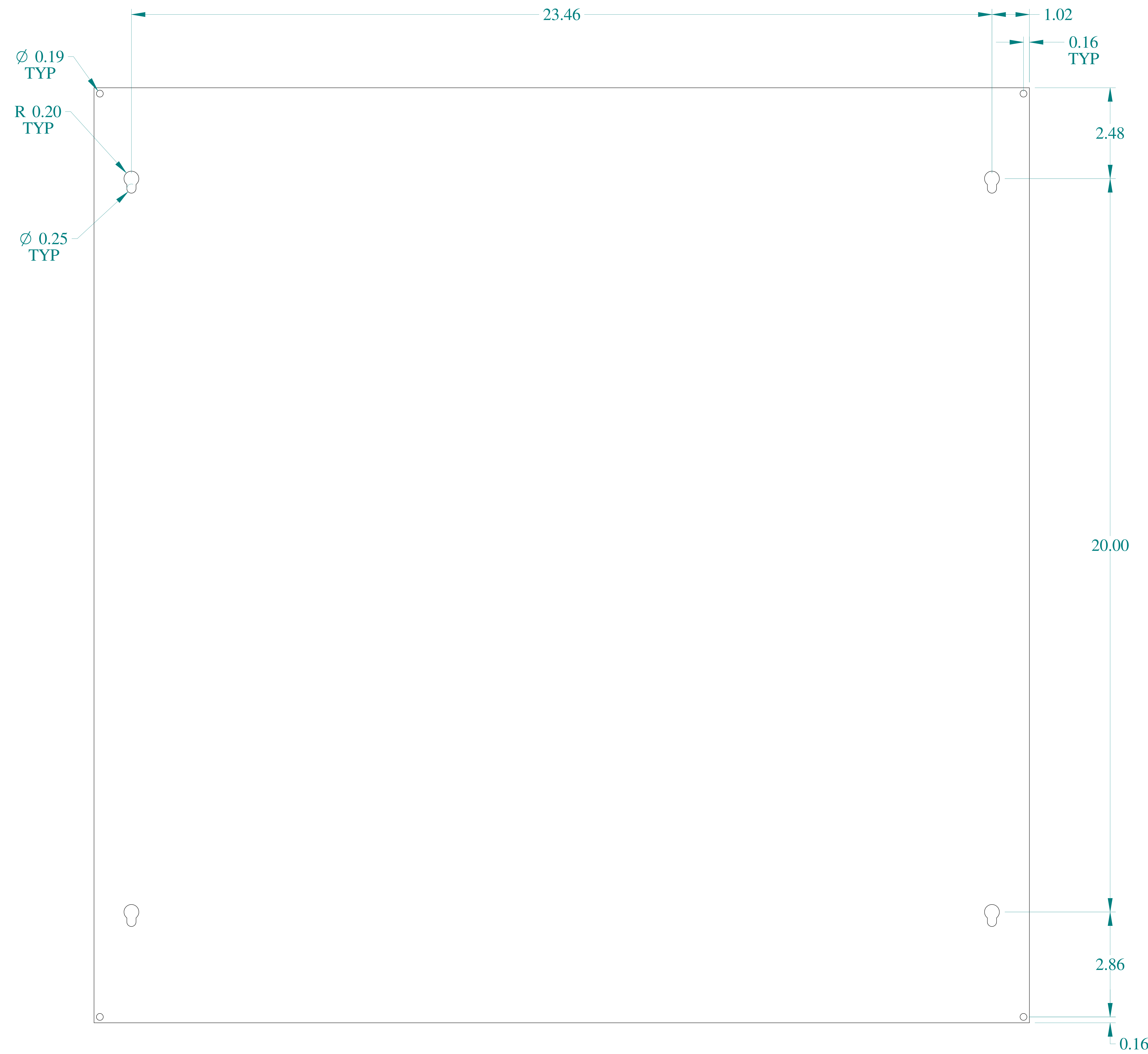
FRONT VIEW
