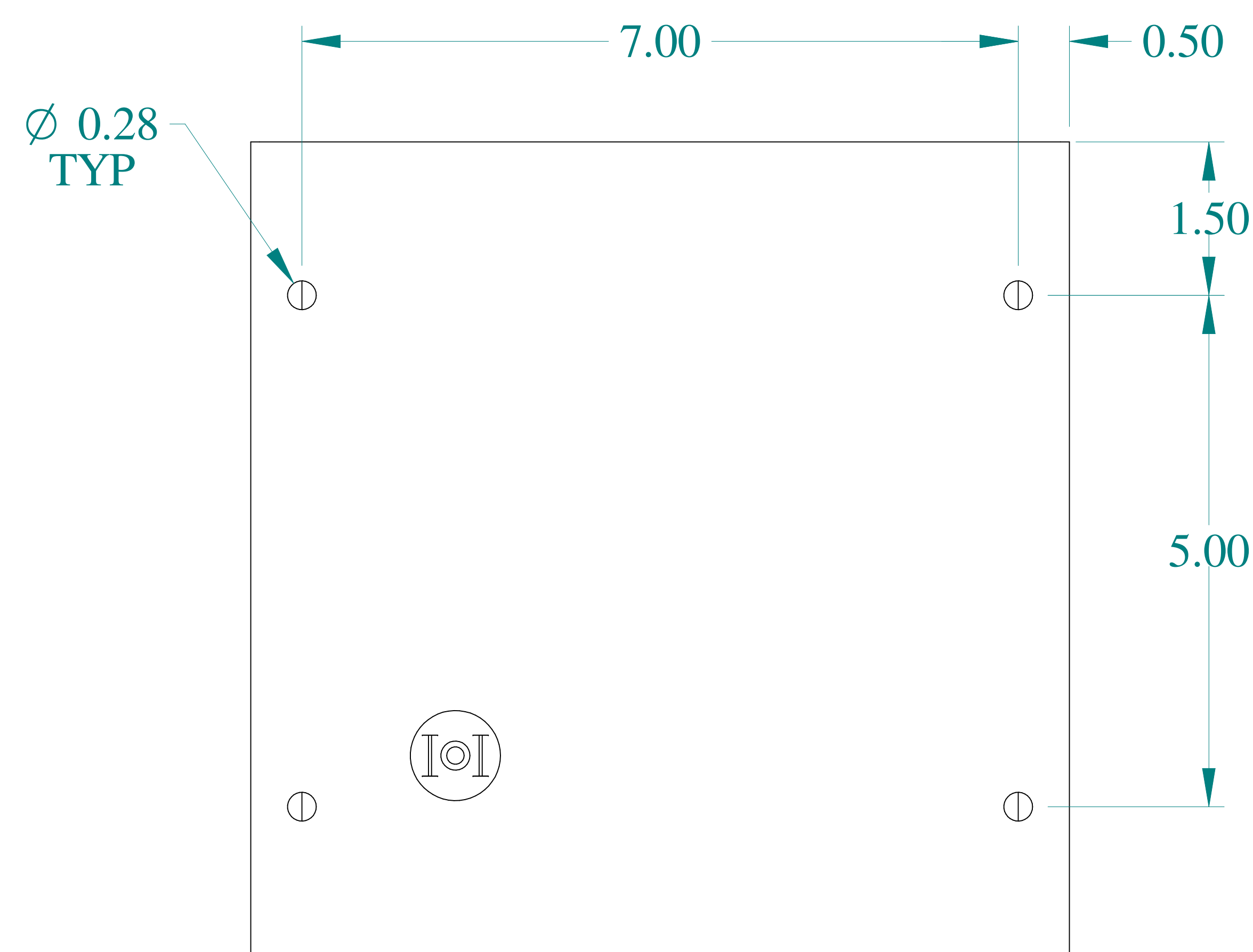
BOTTOM VIEW
