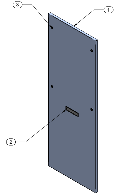
ISOMETRIC
