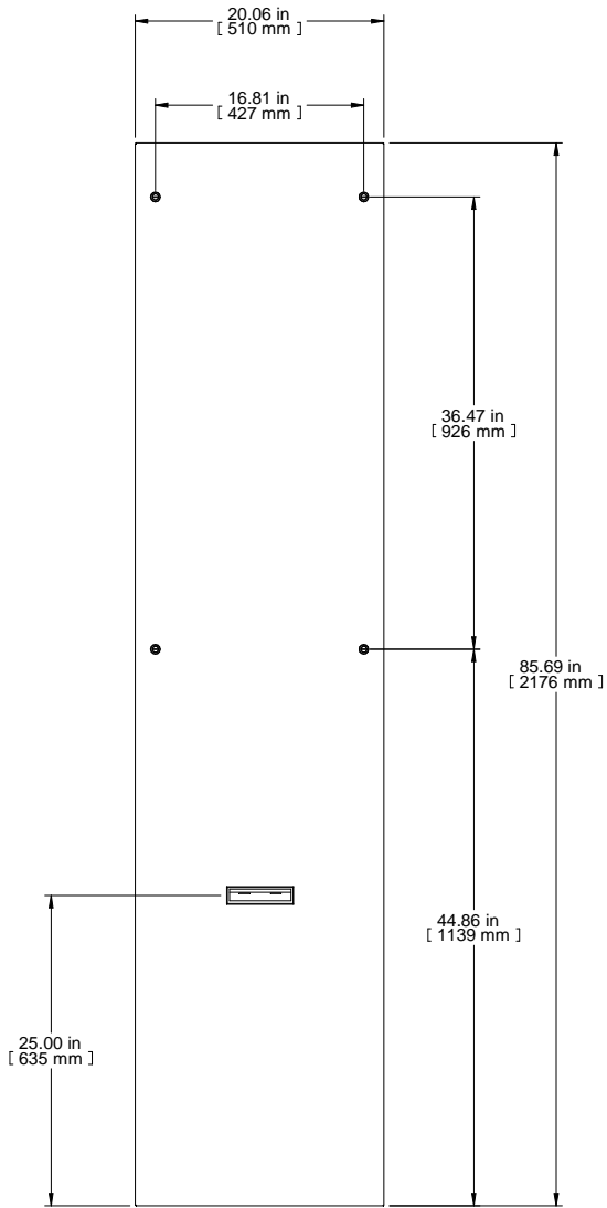
FRONT VIEW
