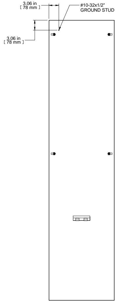
REAR VIEW
