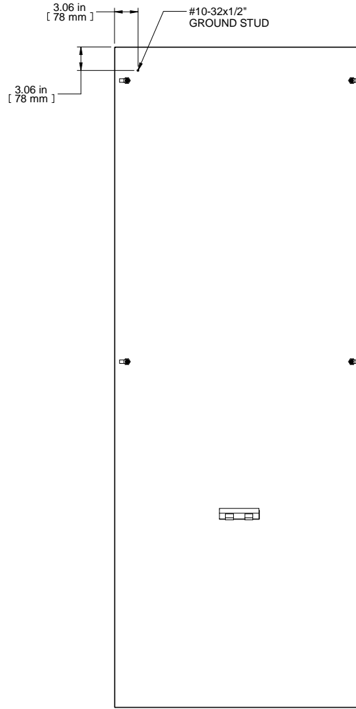
REAR VIEW
