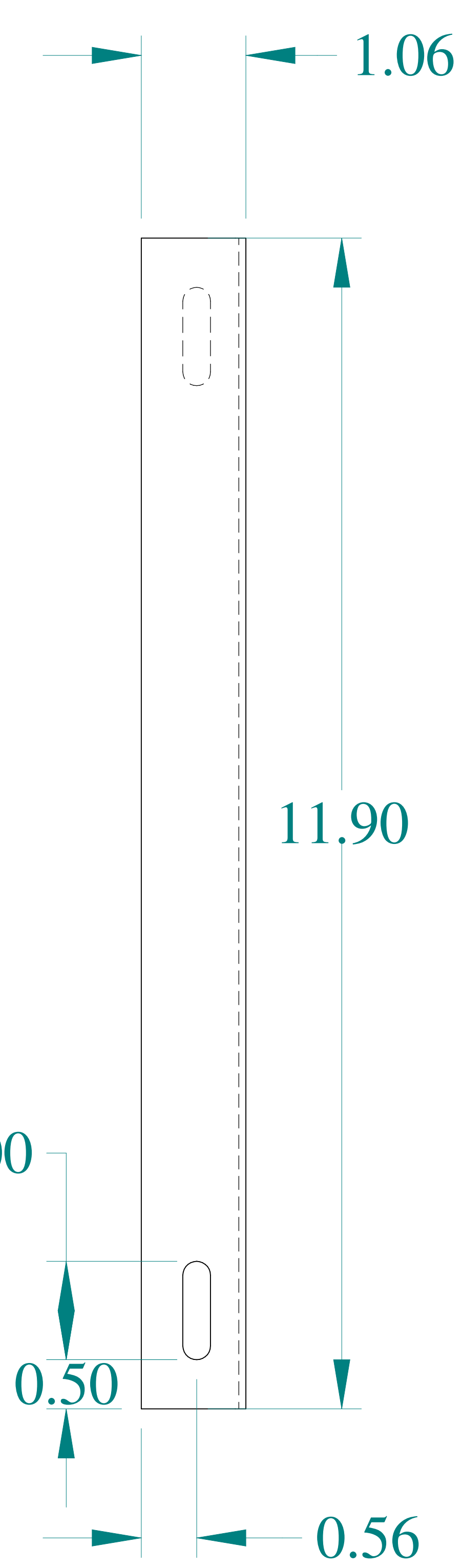
SIDE VIEW
