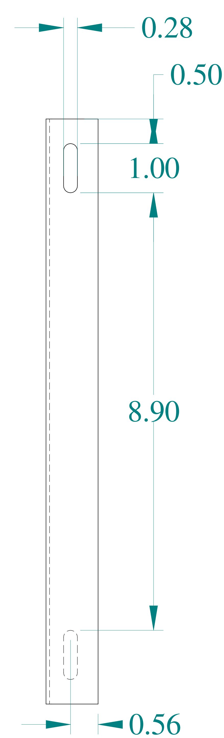
SIDE VIEW
