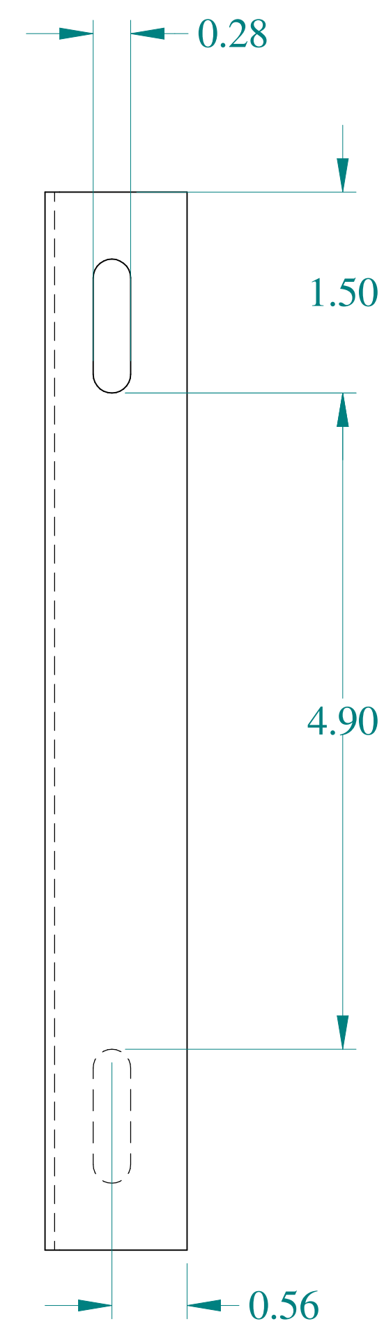
SIDE VIEW
