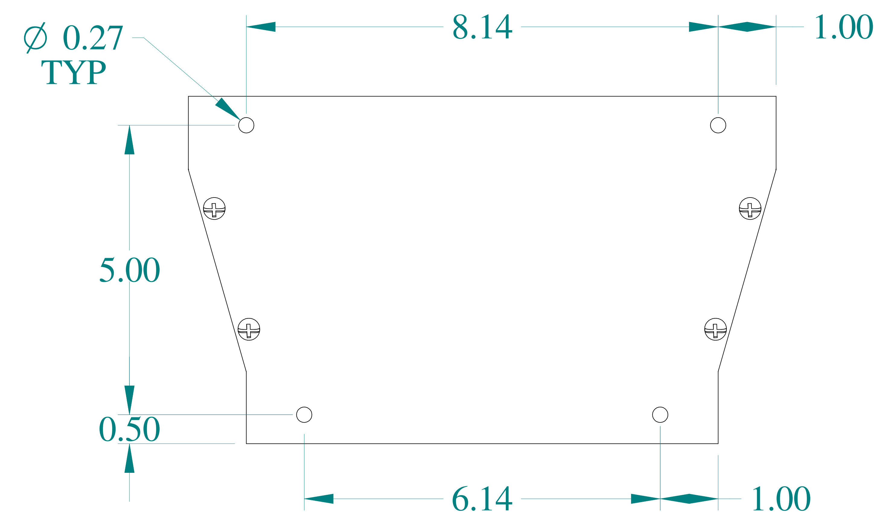
TOP VIEW
