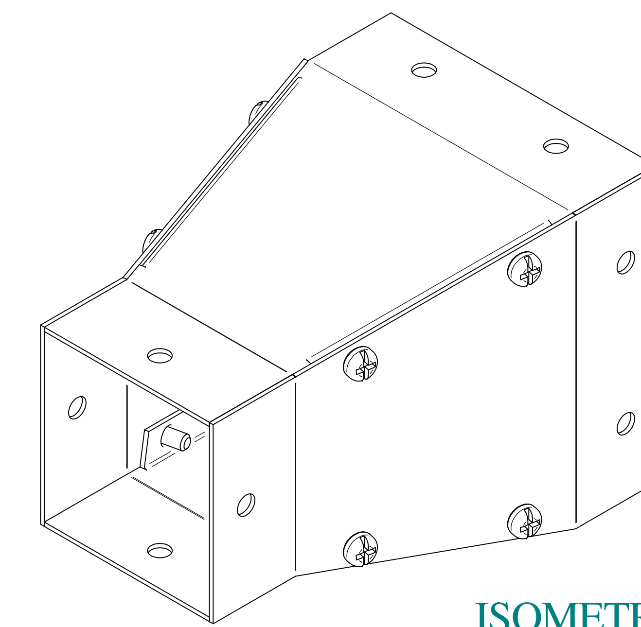
ISOMETRIC VIEWS
