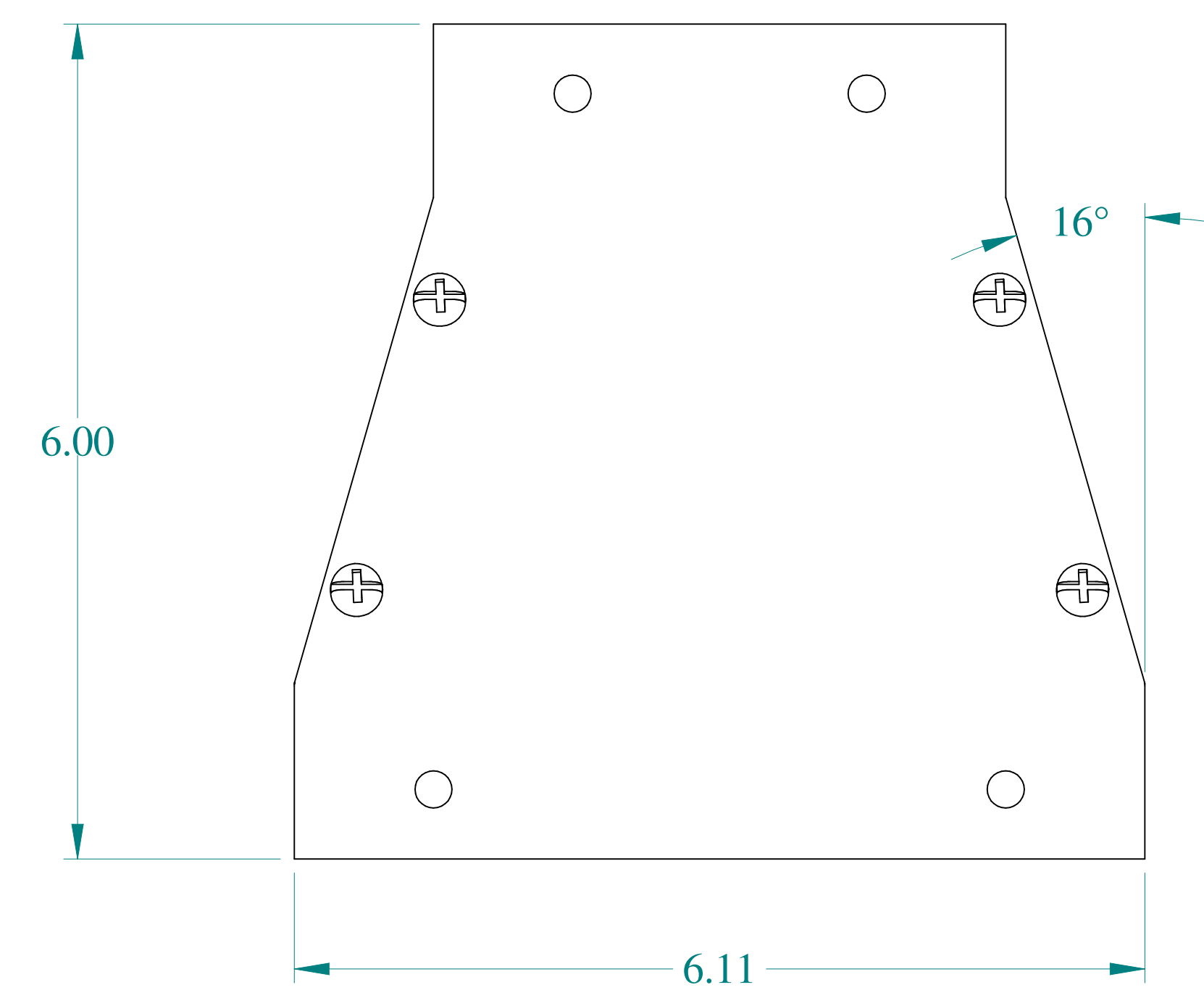
BOTTOM VIEW
