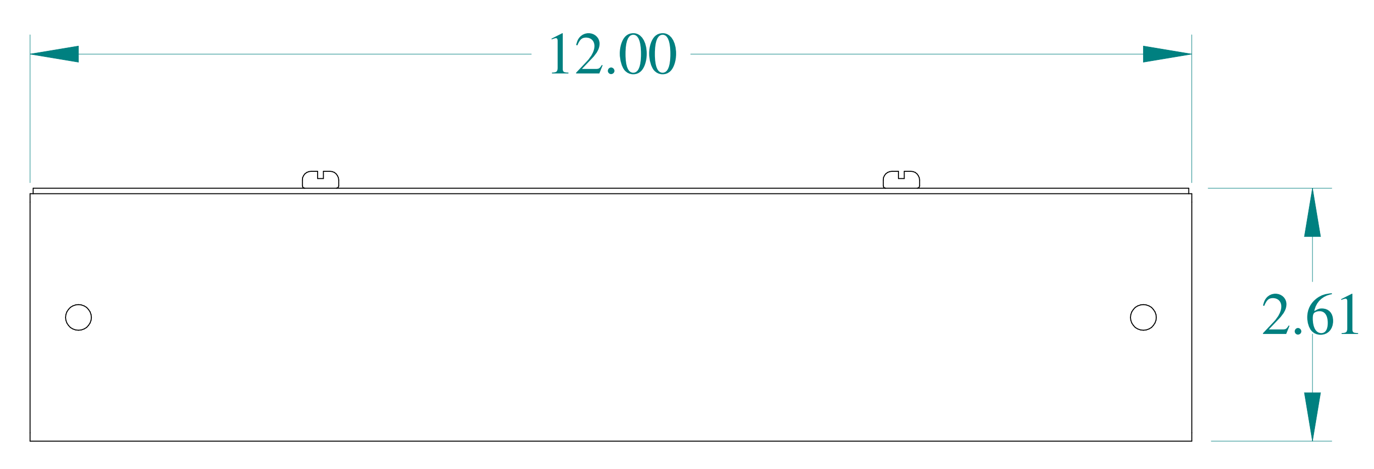
SIDE VIEW
