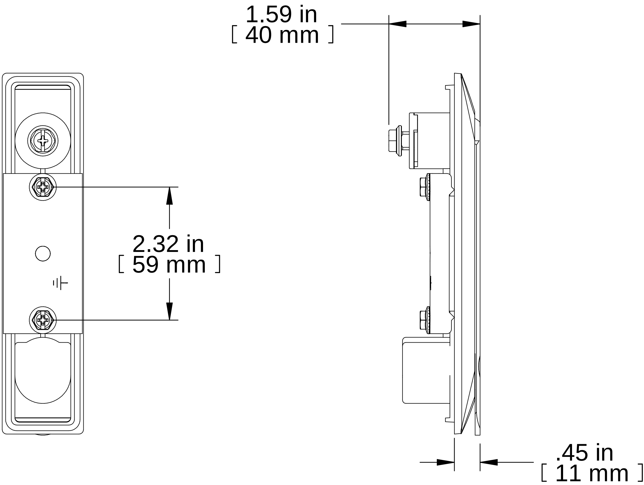
REAR VIEW
