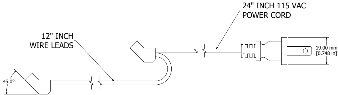
SIDE VIEW
