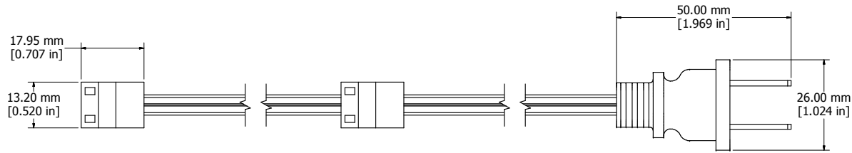
BOTTOM VIEW
