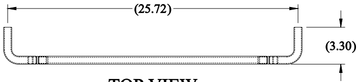
TOP VIEW
