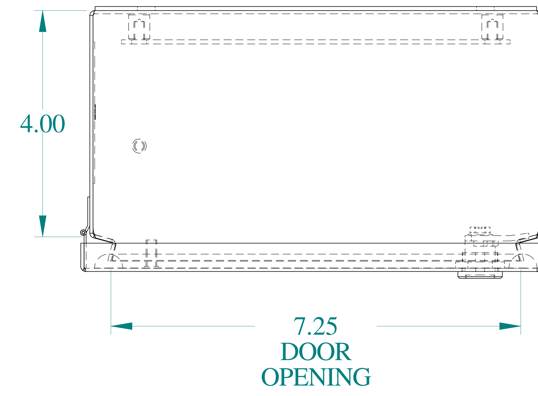
TOP VIEW
