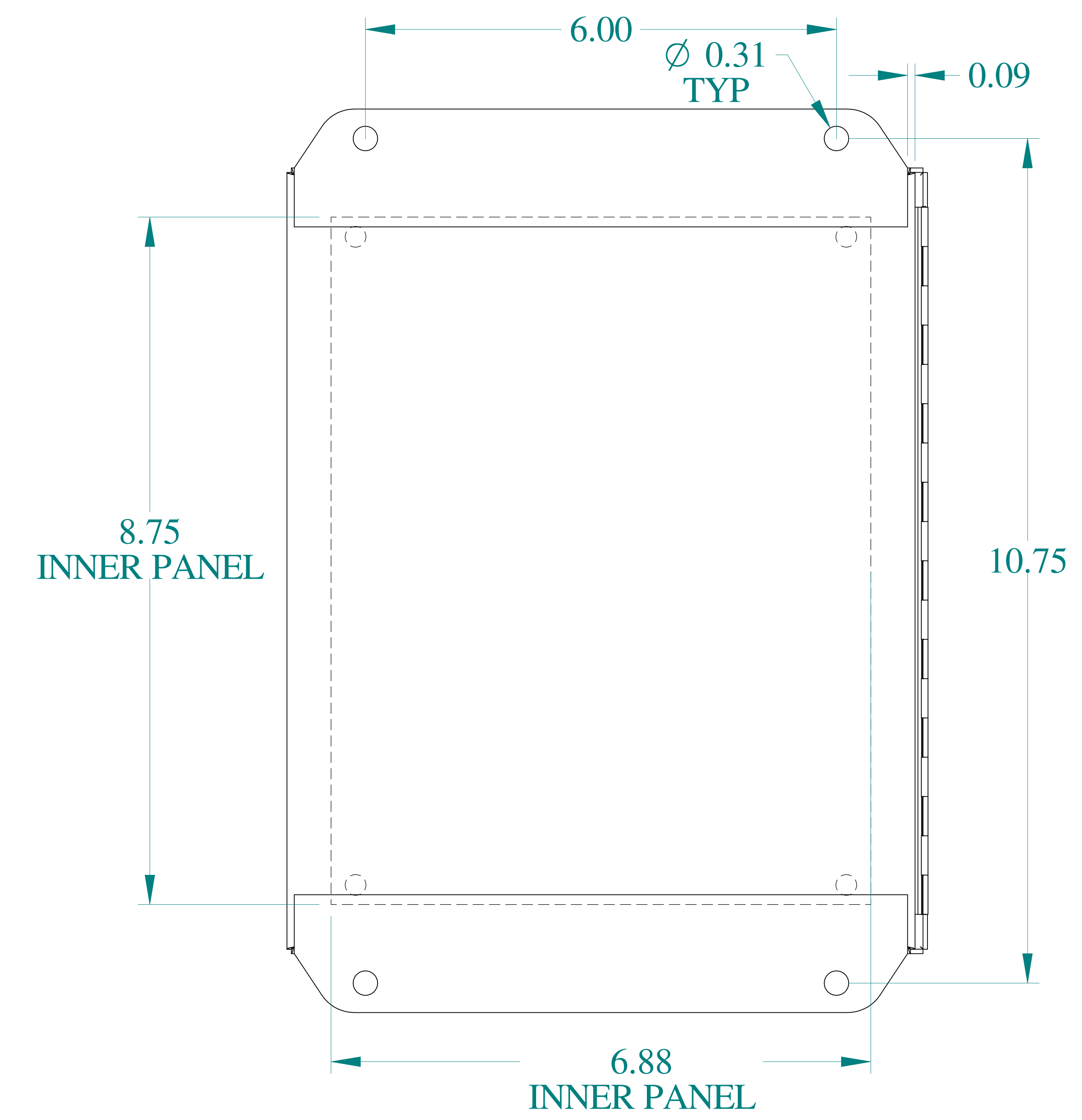
BACK VIEW
