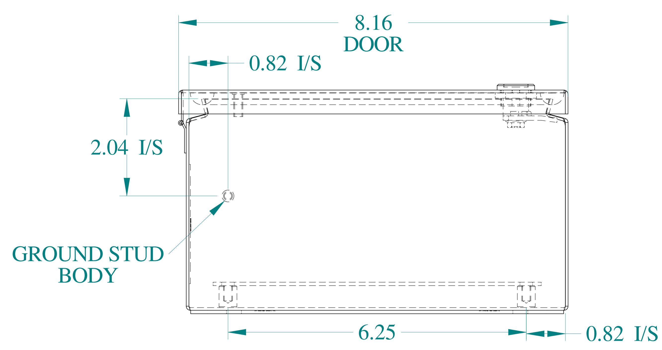
BOTTOM VIEW
