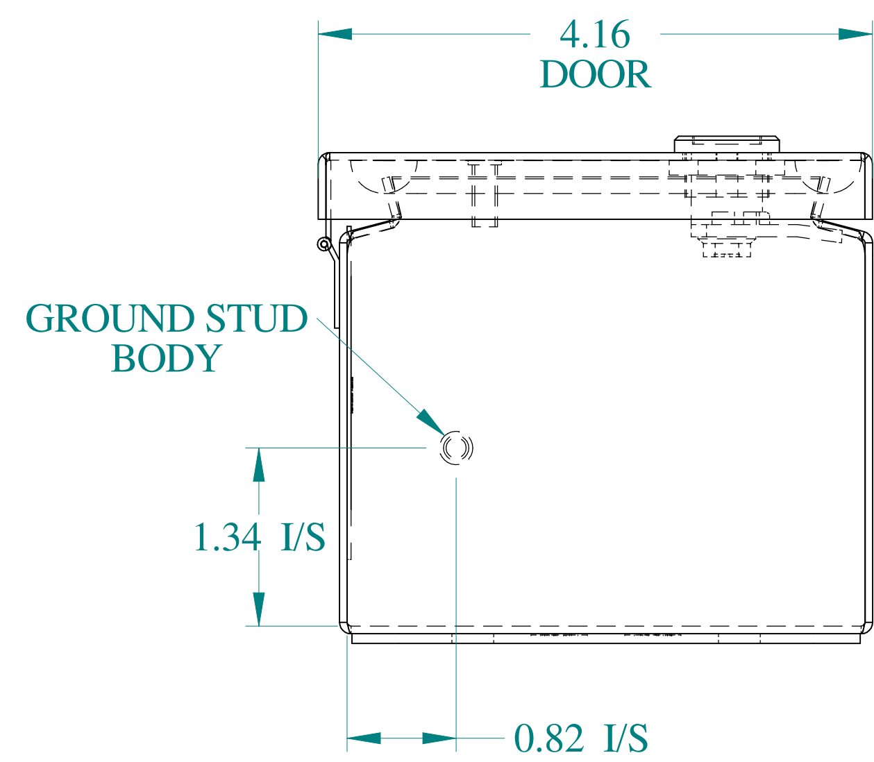
BOTTOM VIEW
