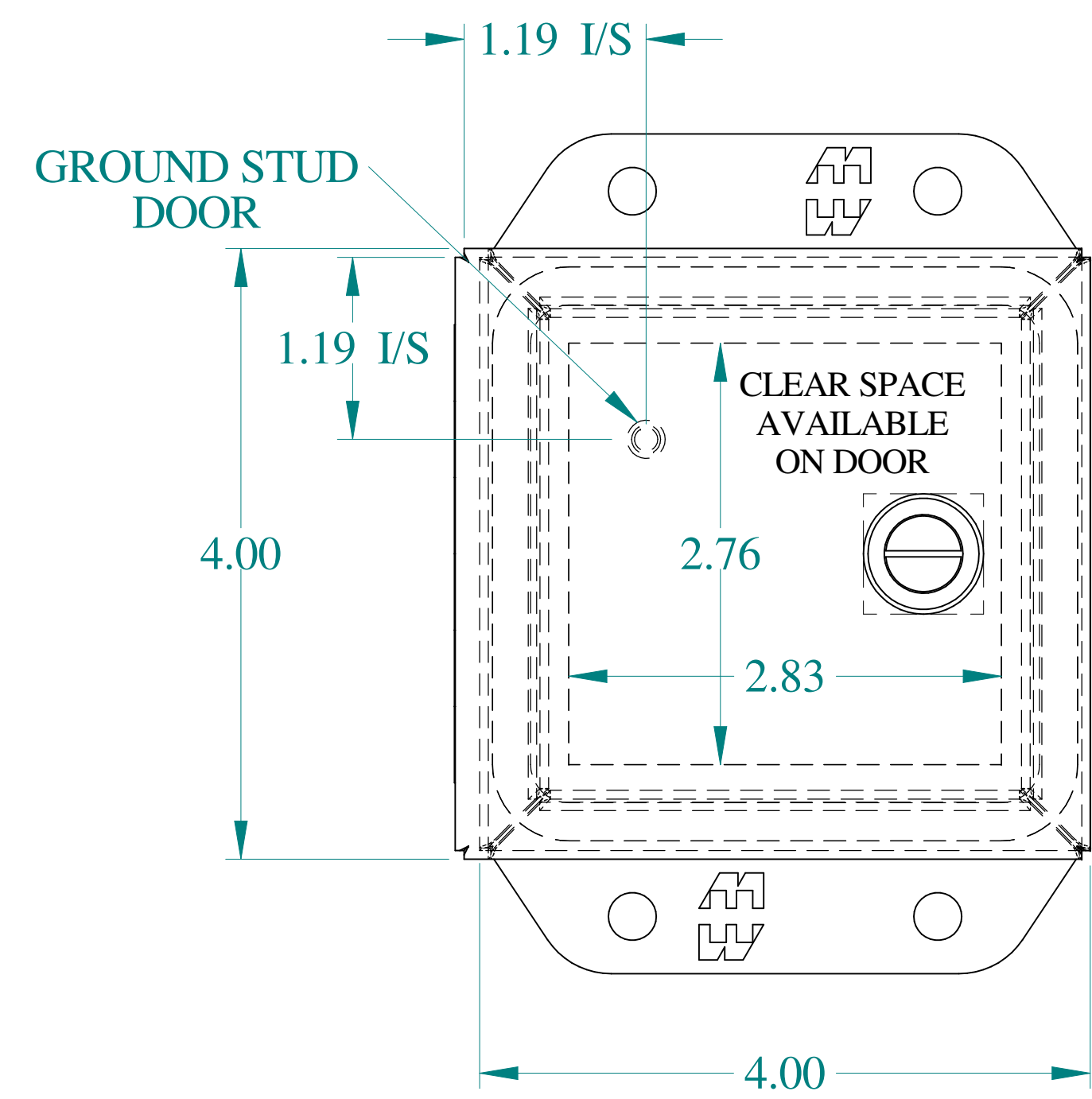
FRONT VIEW
