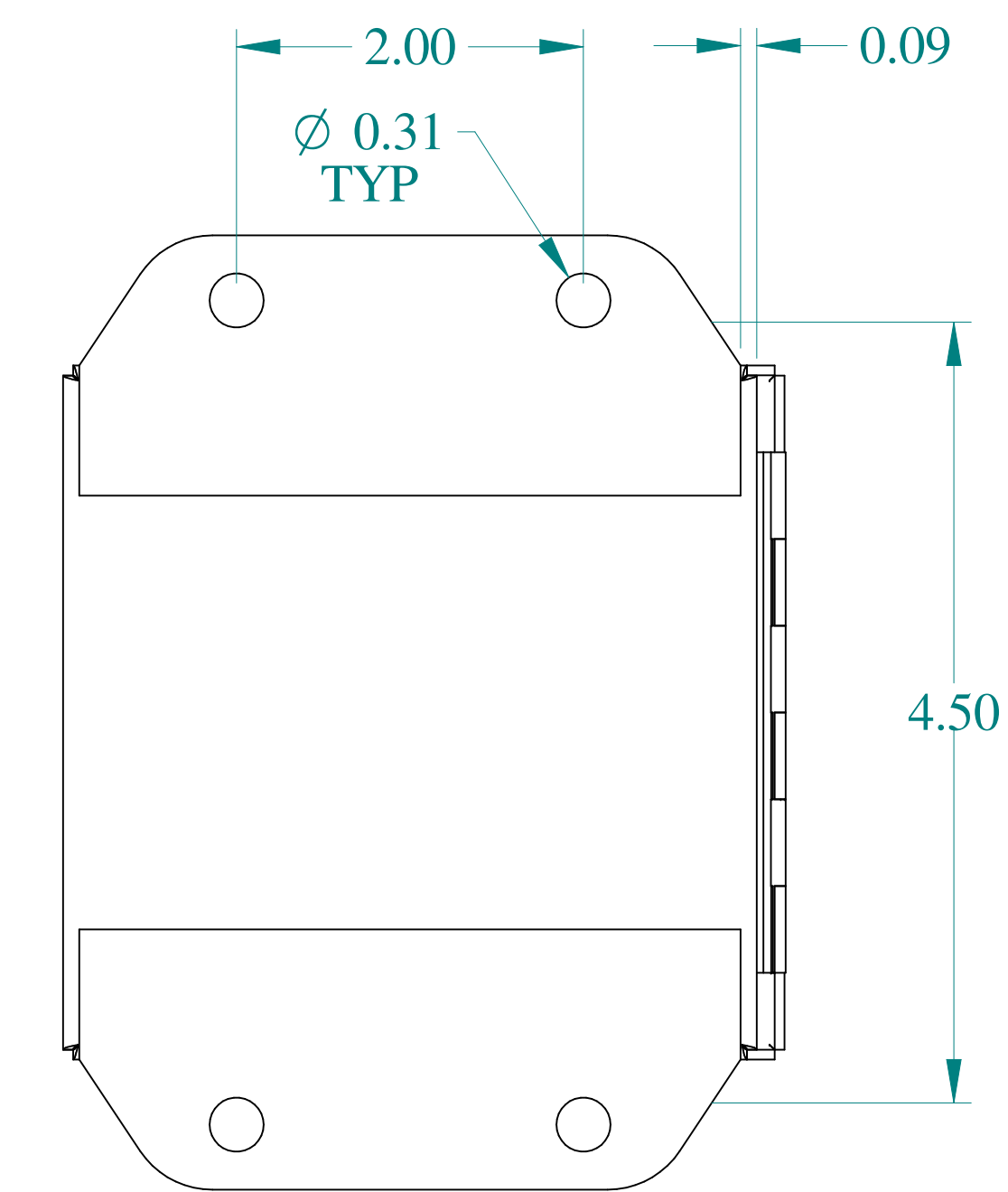
BACK VIEW
