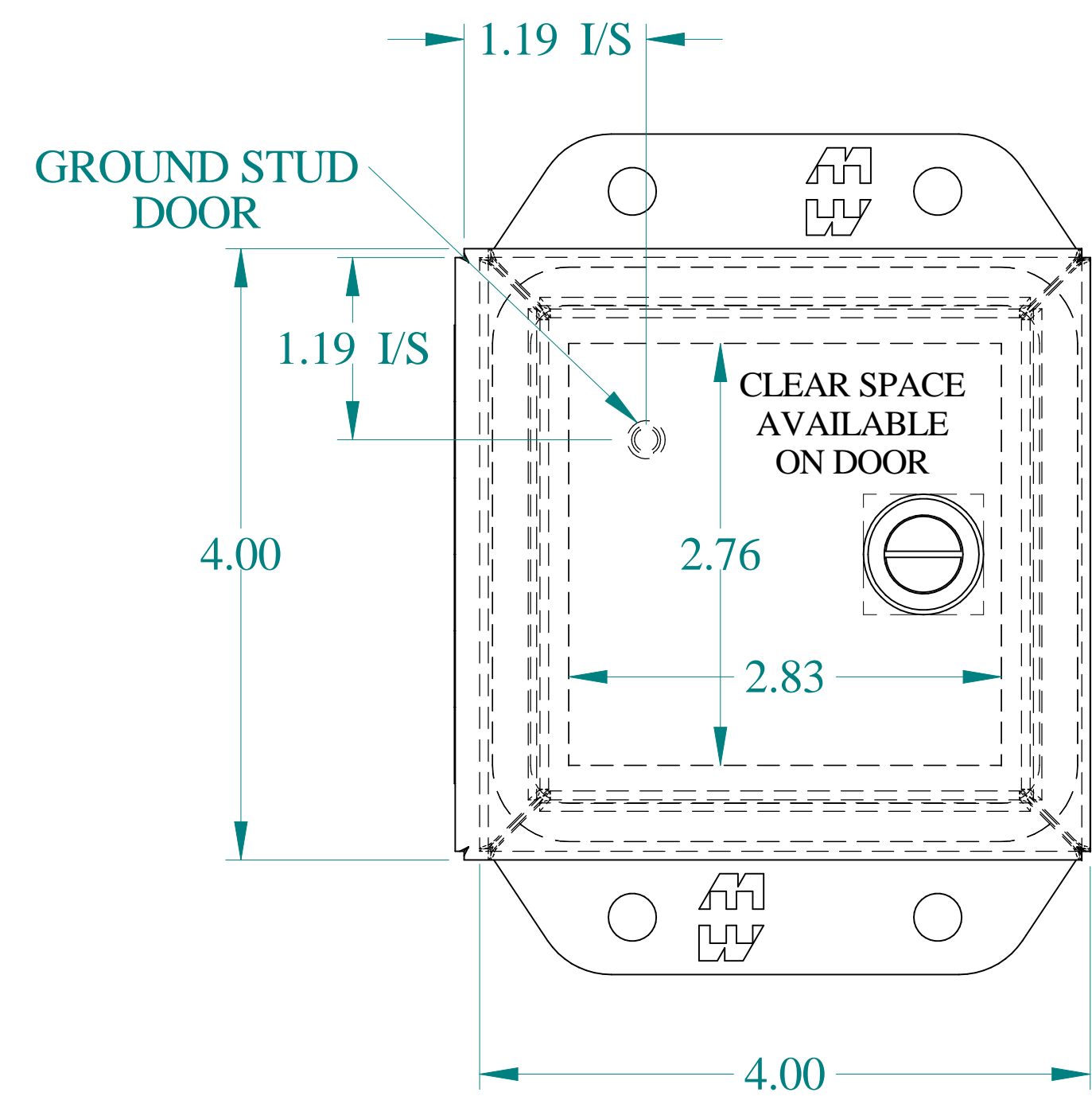
FRONT VIEW
