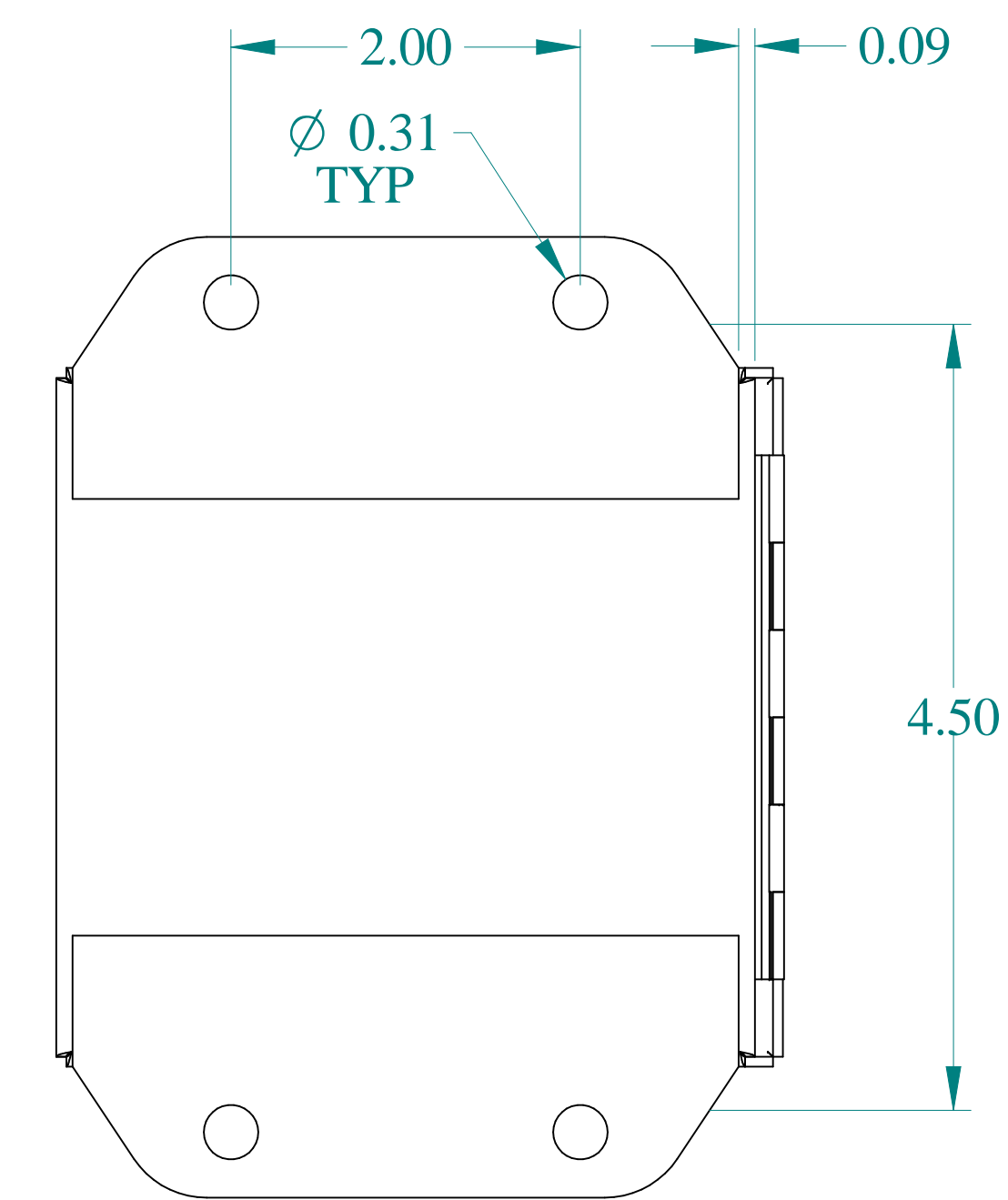
BACK VIEW
