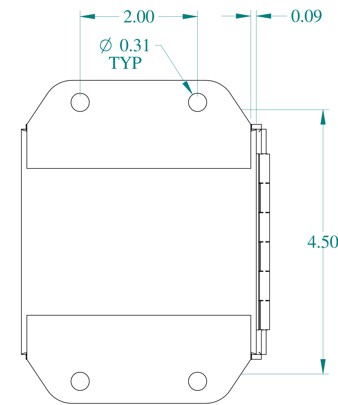
BACK VIEW
