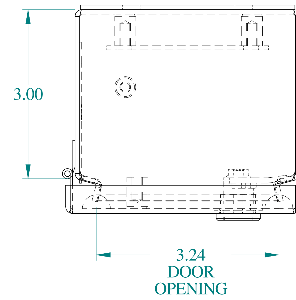
TOP VIEW
