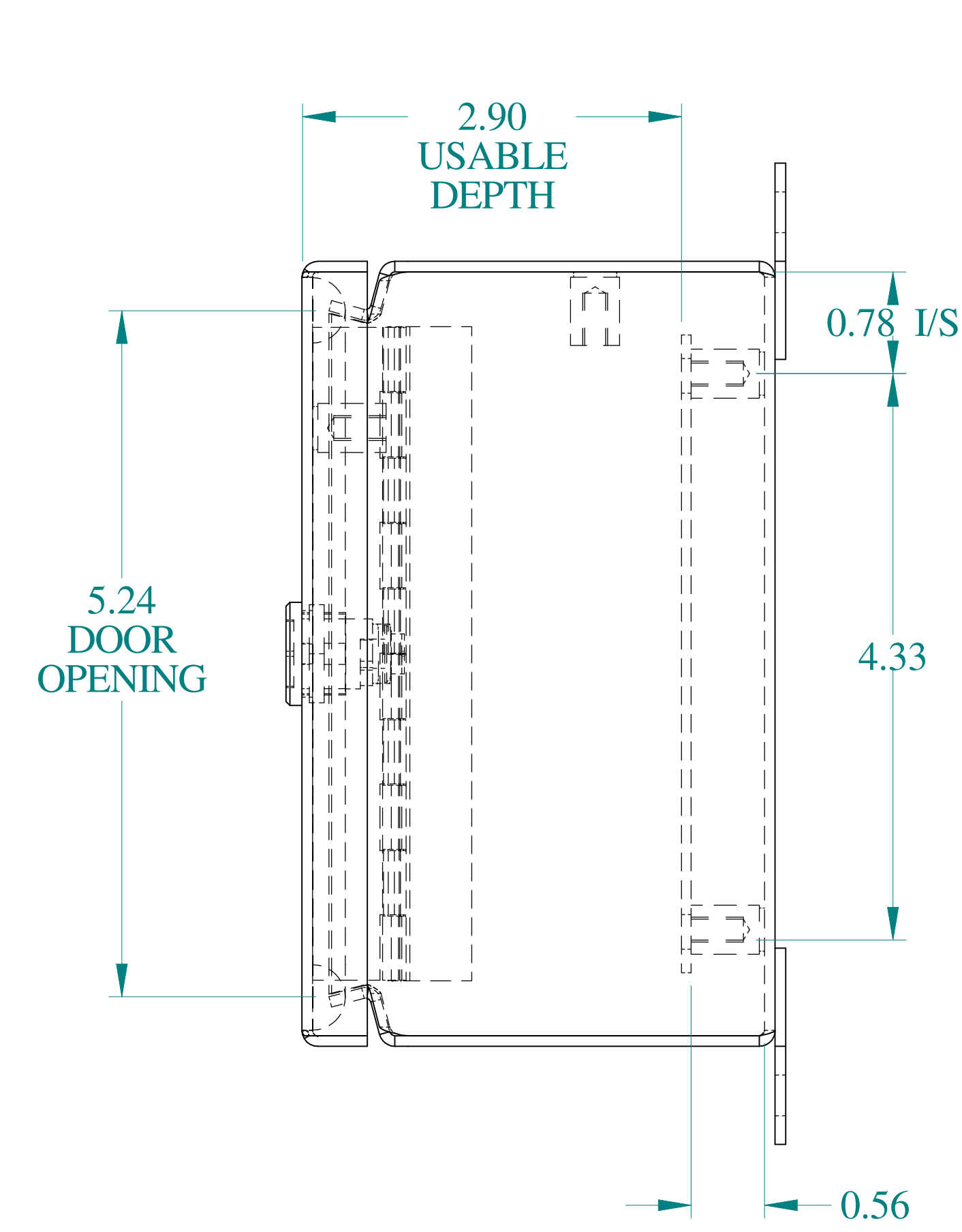
SIDE VIEW
