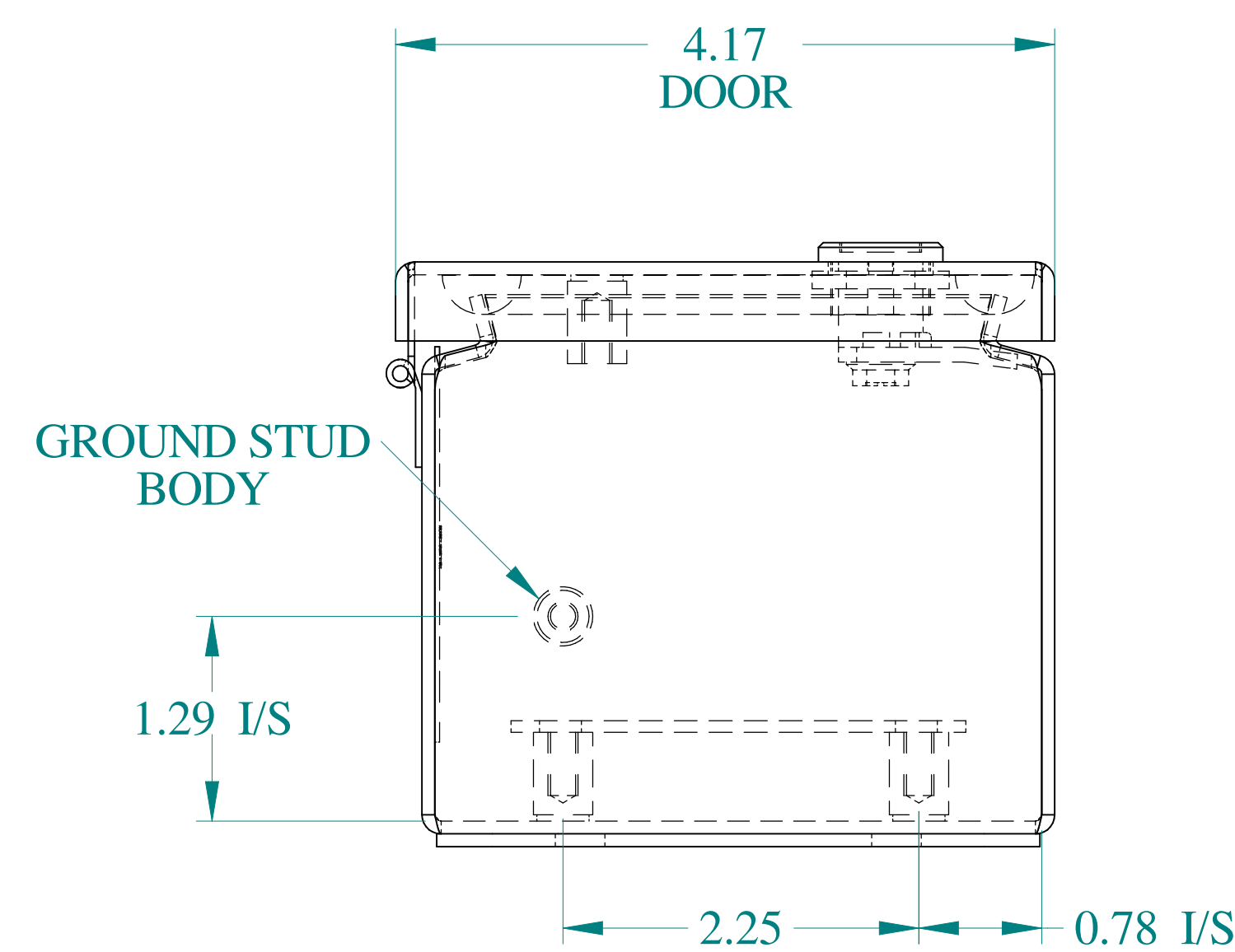
BOTTOM VIEW
