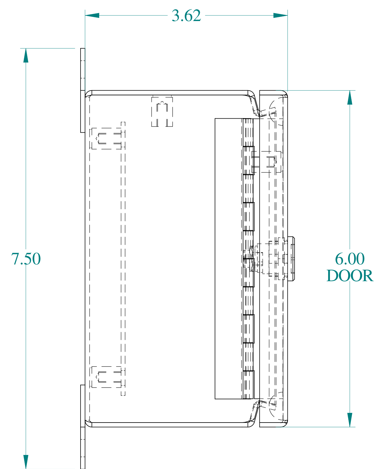
SIDE VIEW
