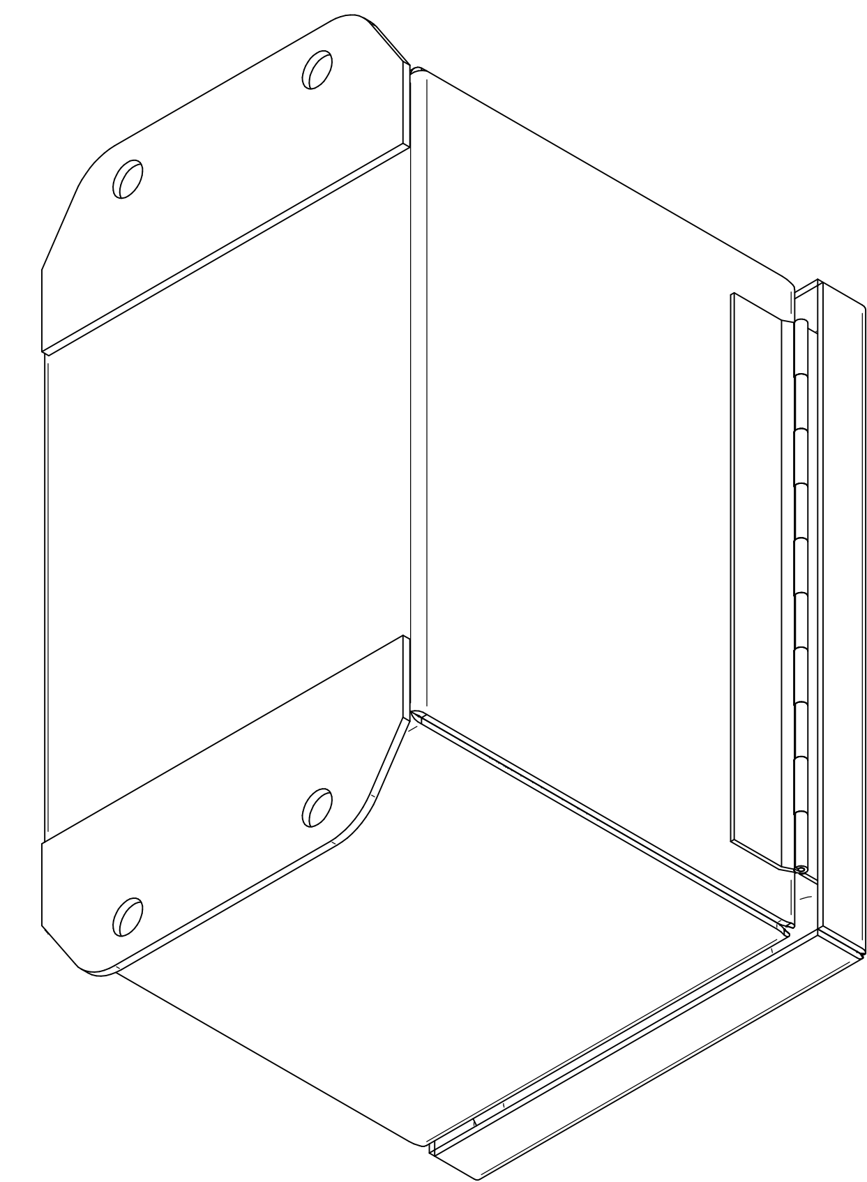
ISOMETRIC VIEWS
