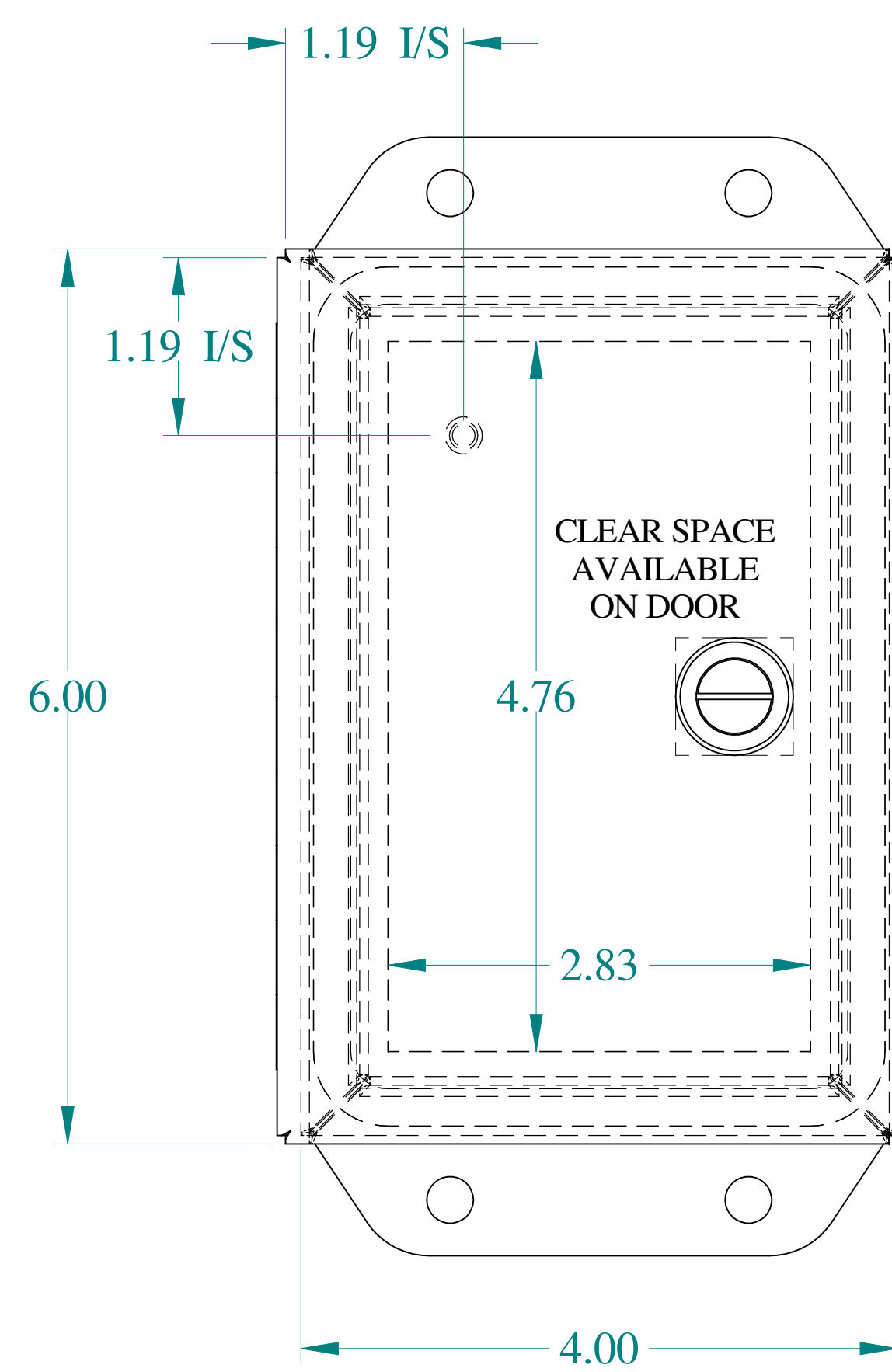
FRONT VIEW
