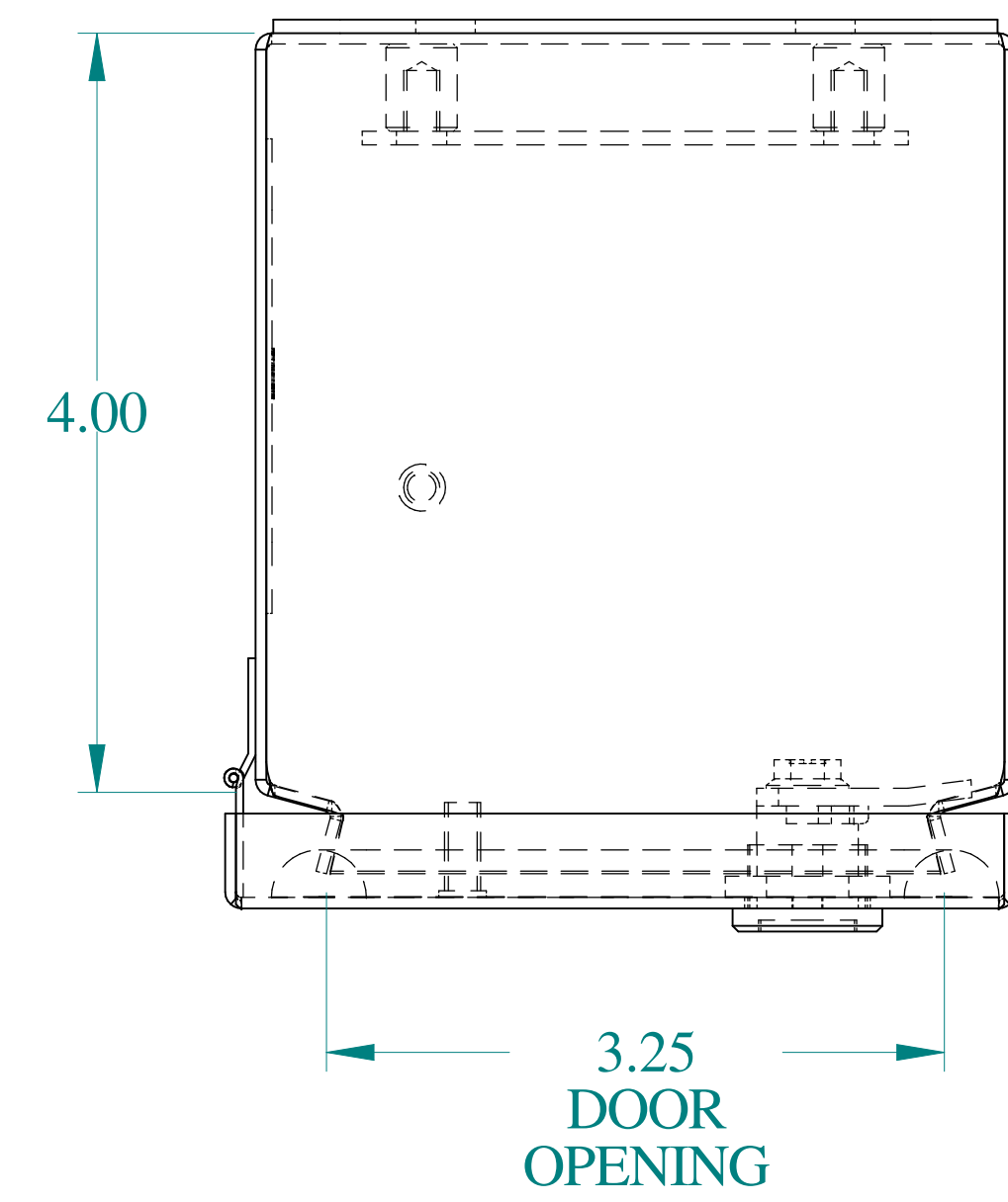
TOP VIEW
