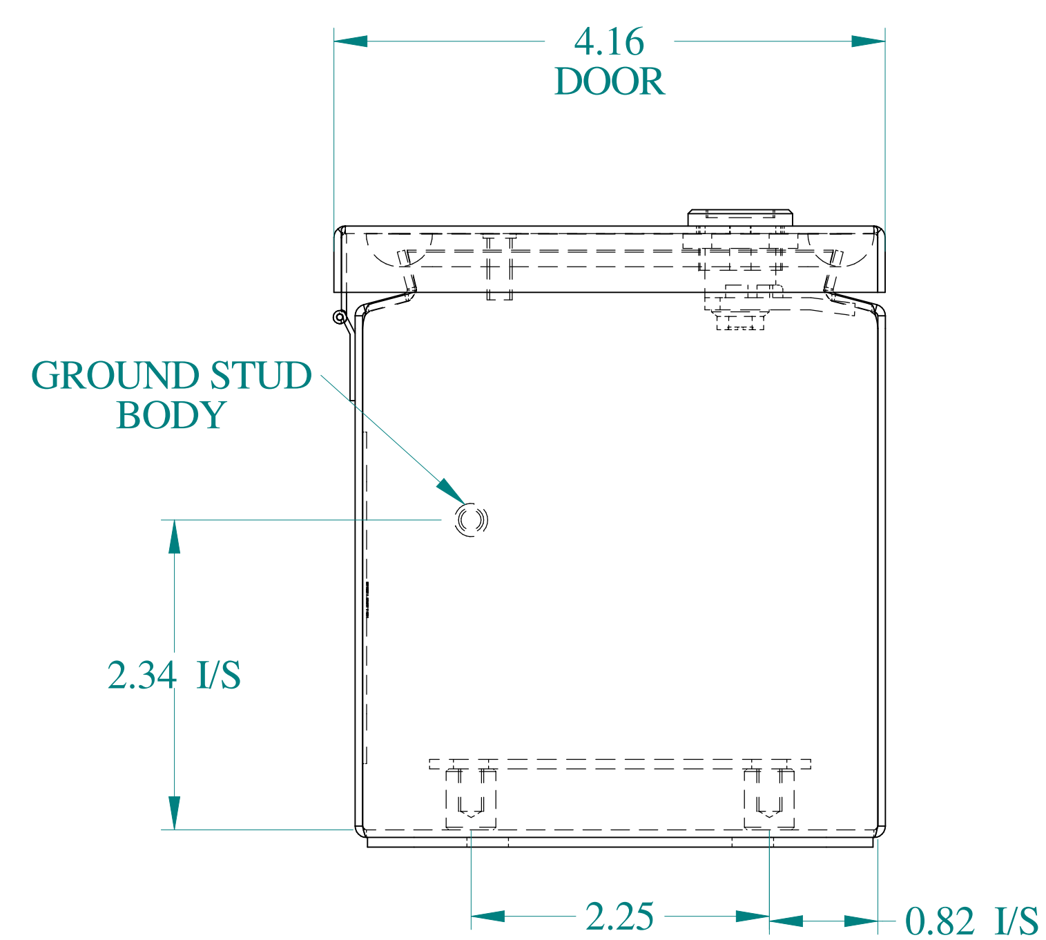
BOTTOM VIEW
