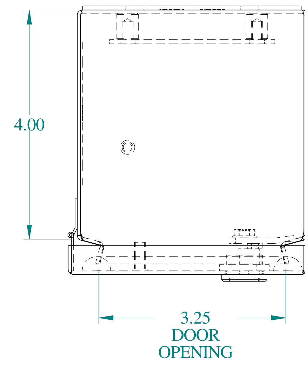
TOP VIEW
