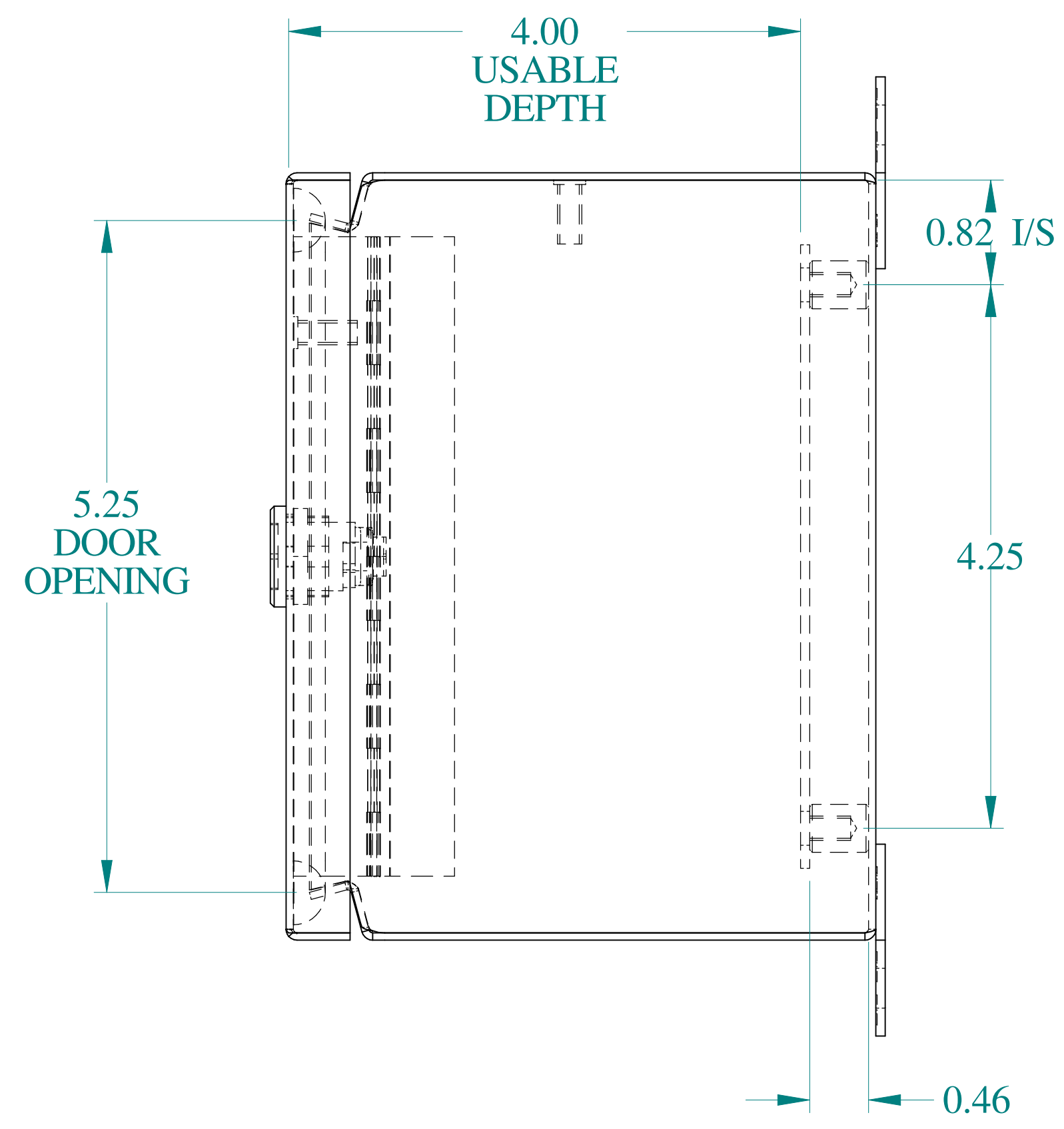
SIDE VIEW
