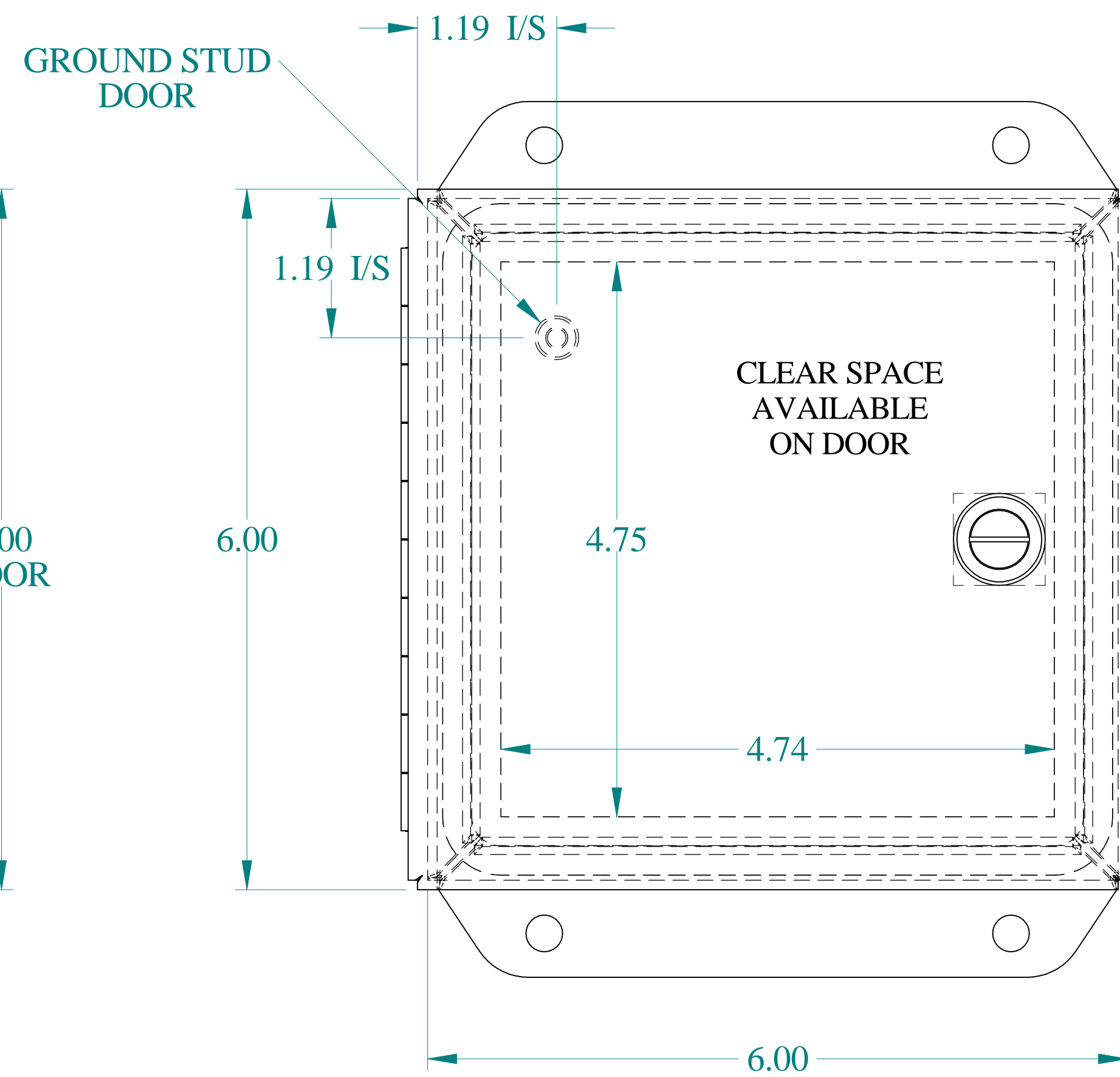
FRONT VIEW
