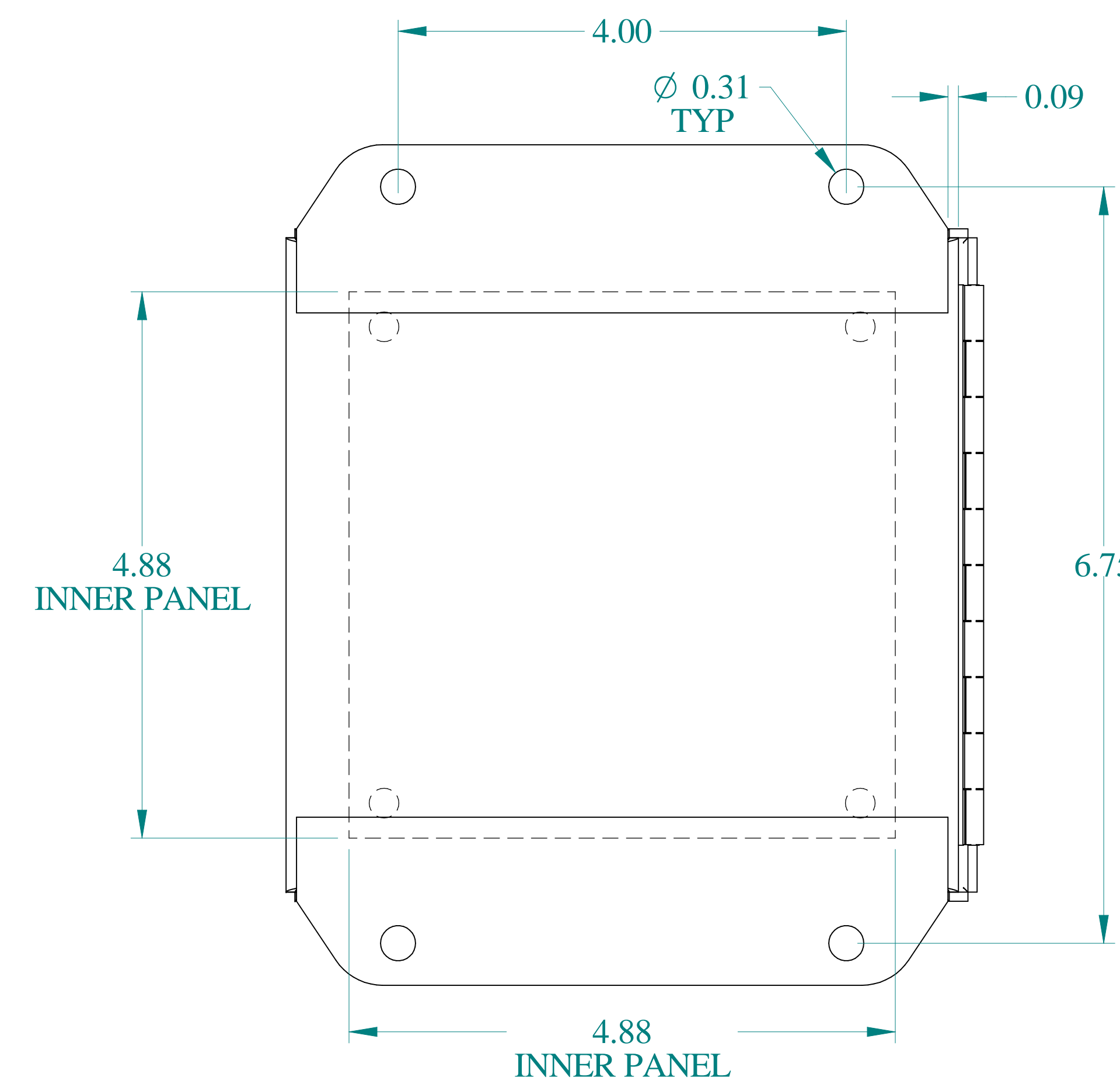
BACK VIEW
