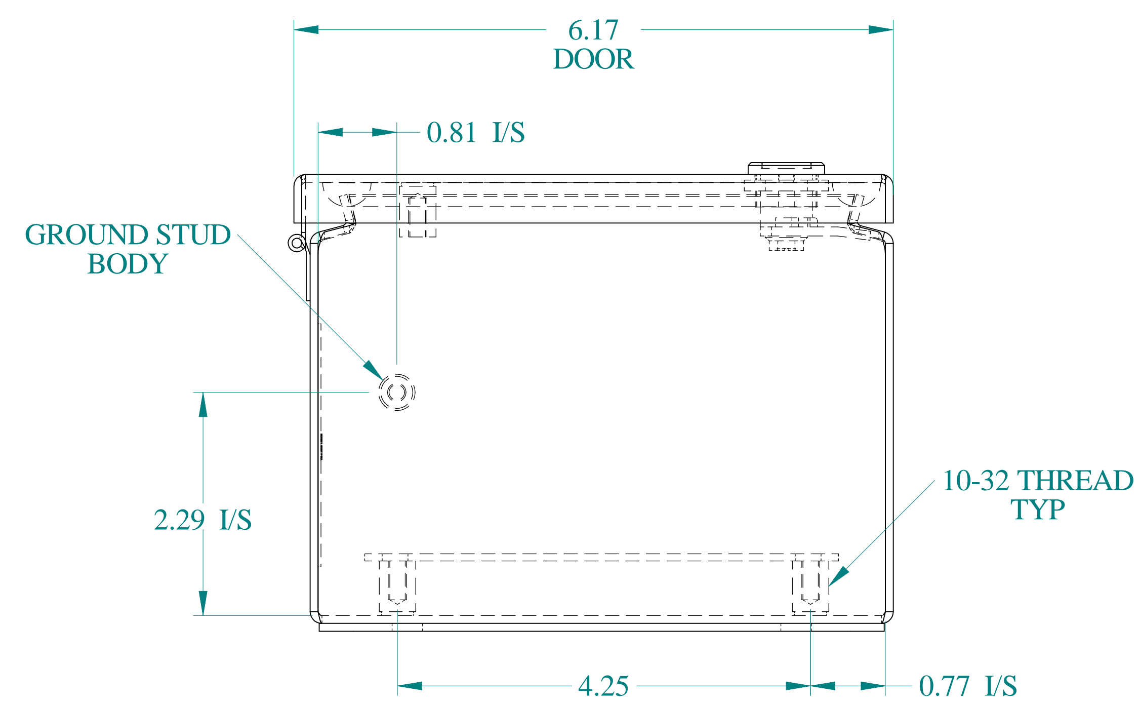
BOTTOM VIEW
