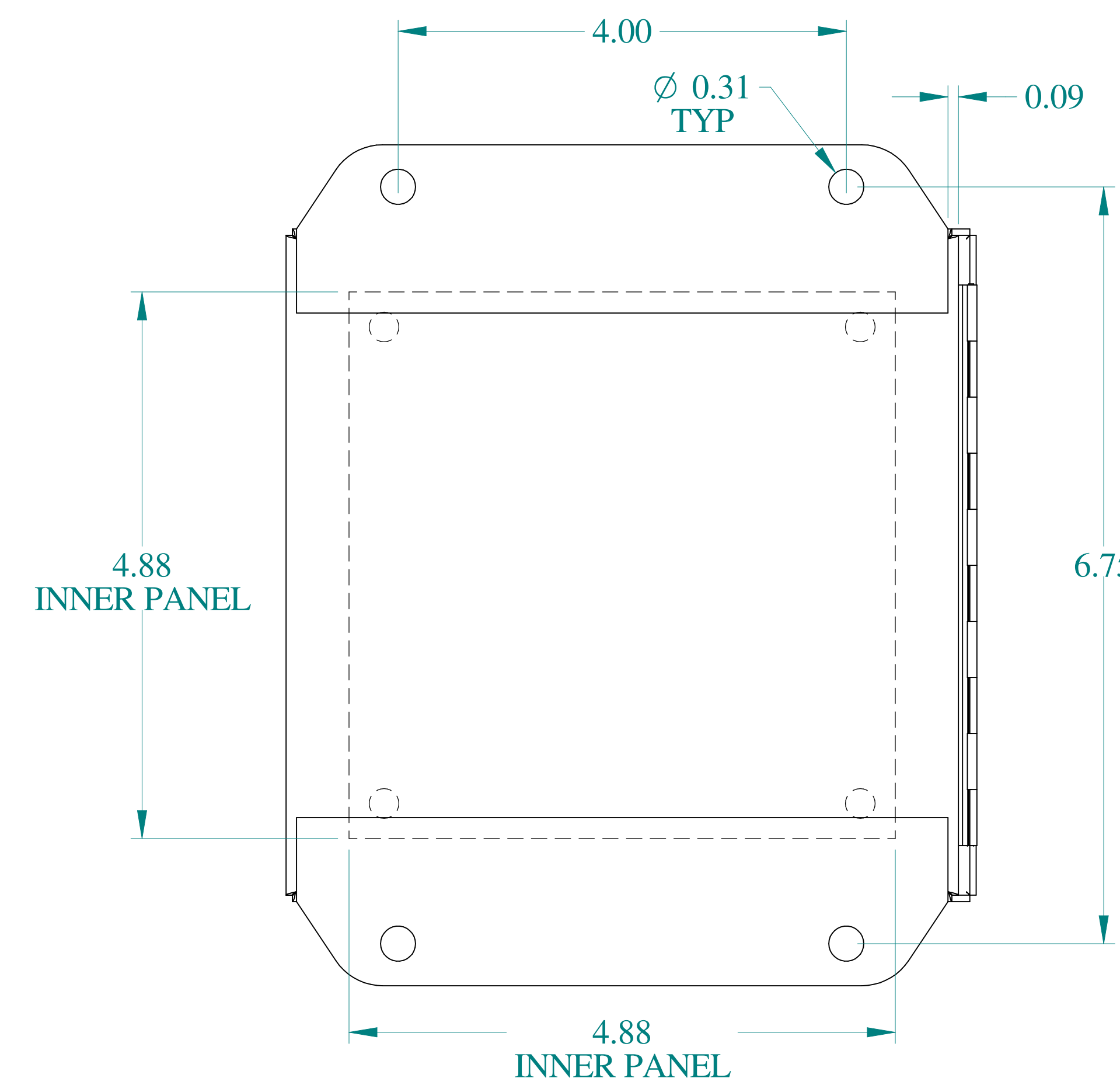
BACK VIEW
