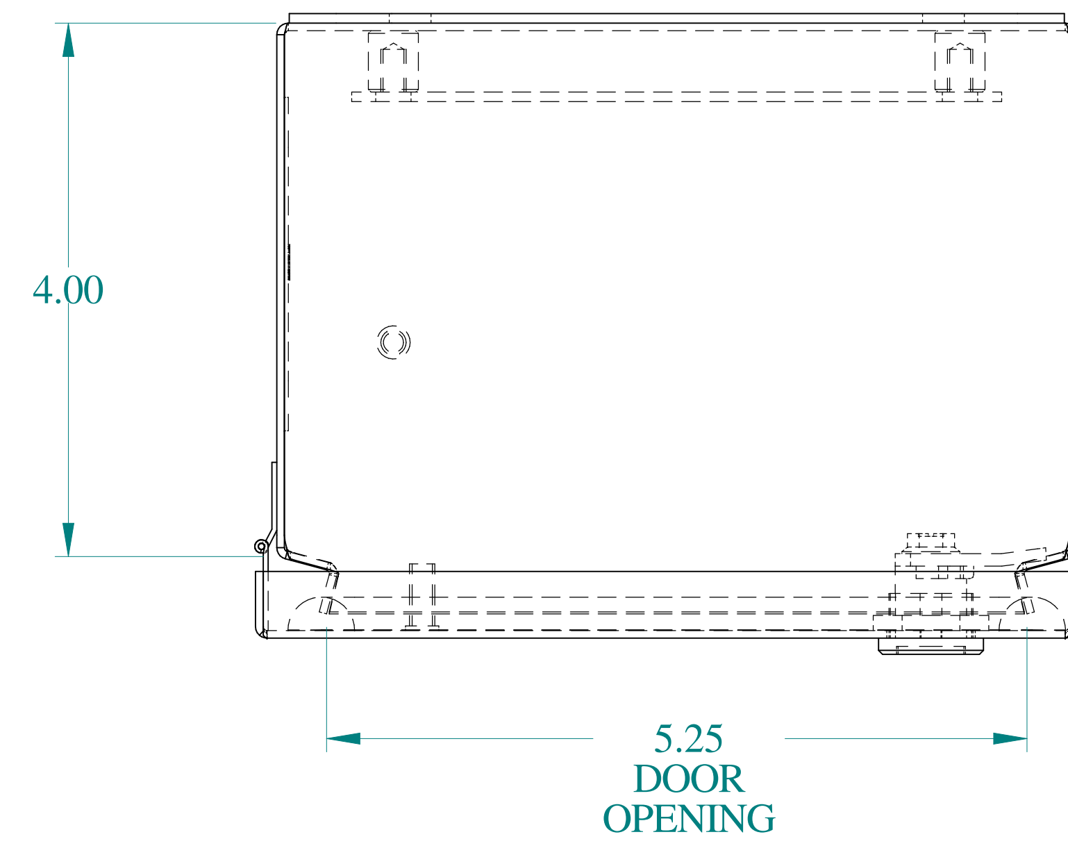
TOP VIEW
