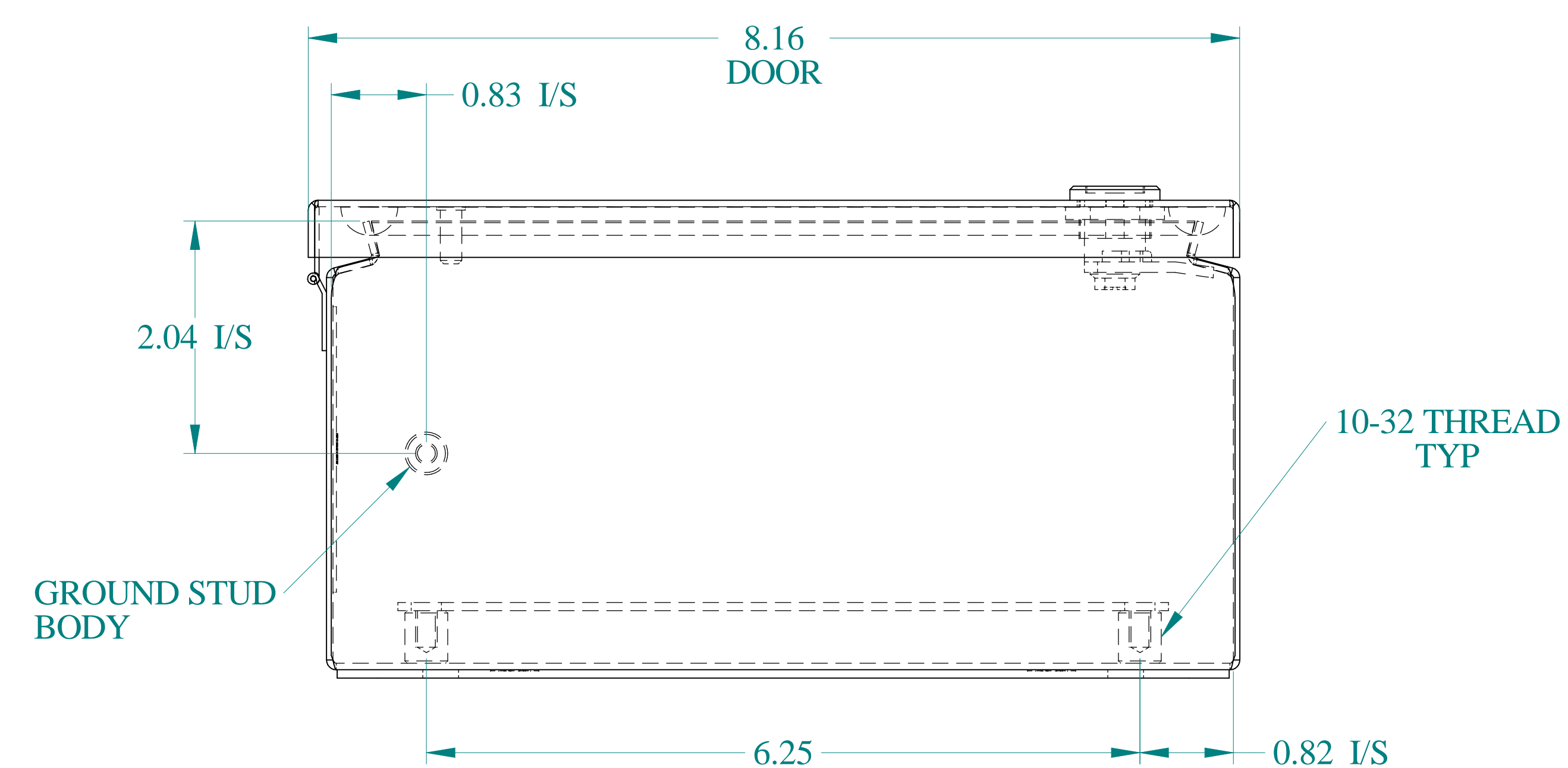
BOTTOM VIEW
