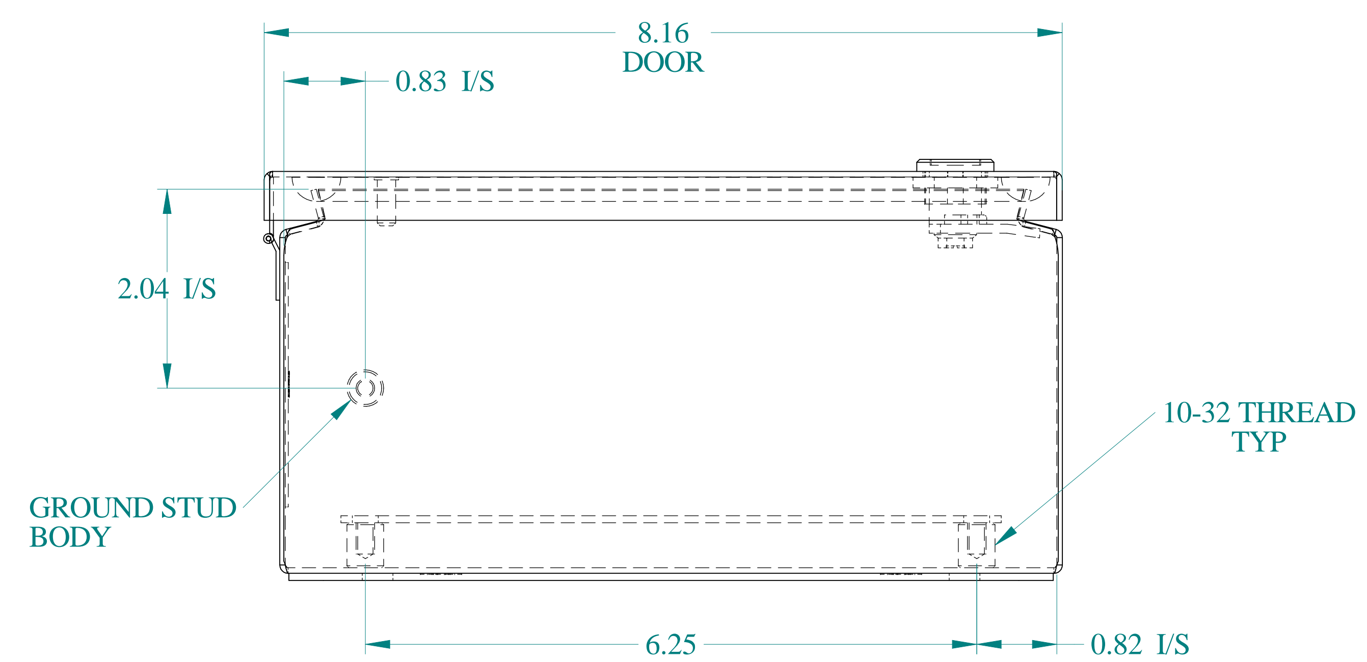
BOTTOM VIEW
