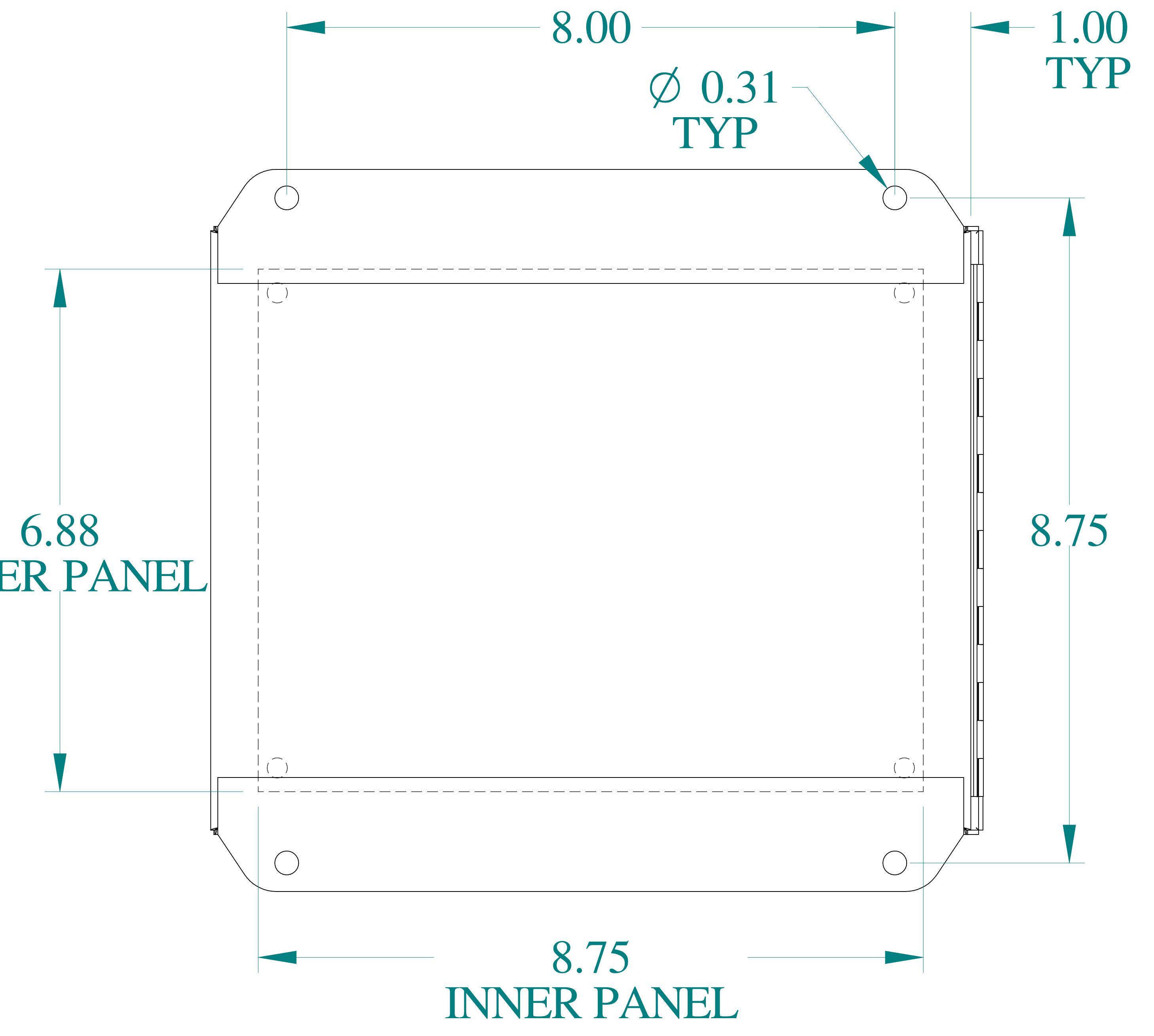
BACK VIEW
