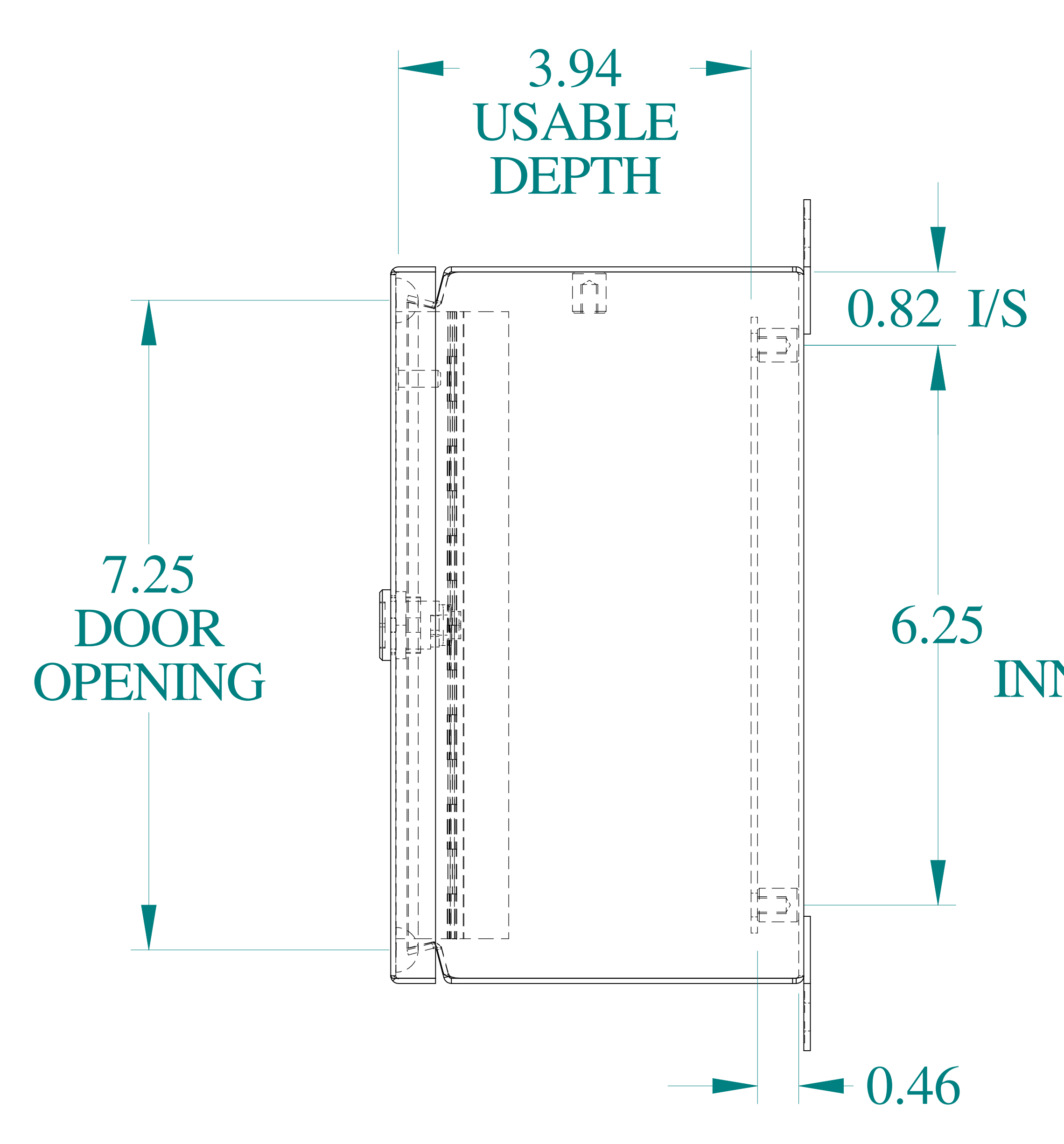
SIDE VIEW
