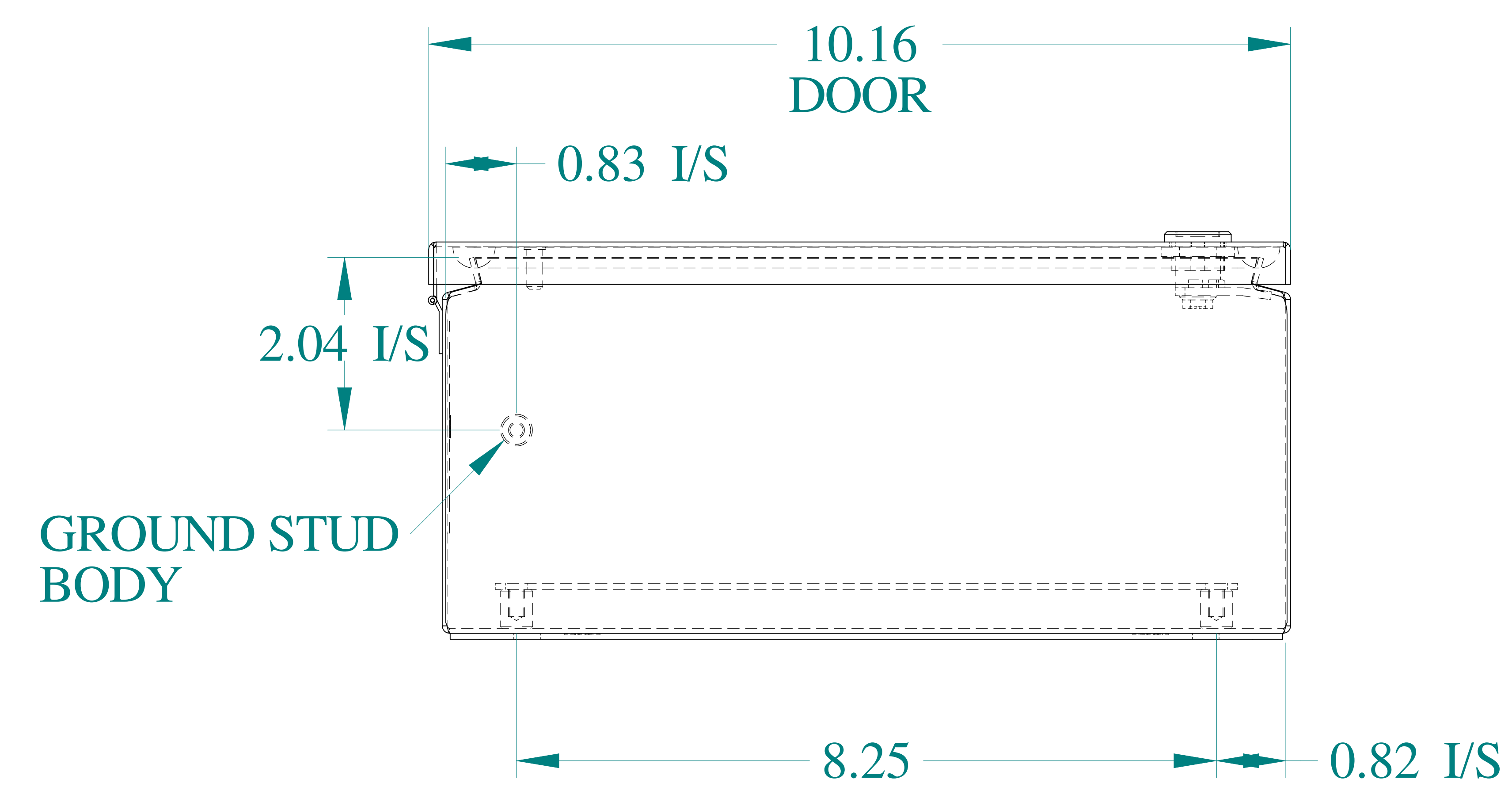
BOTTOM VIEW
