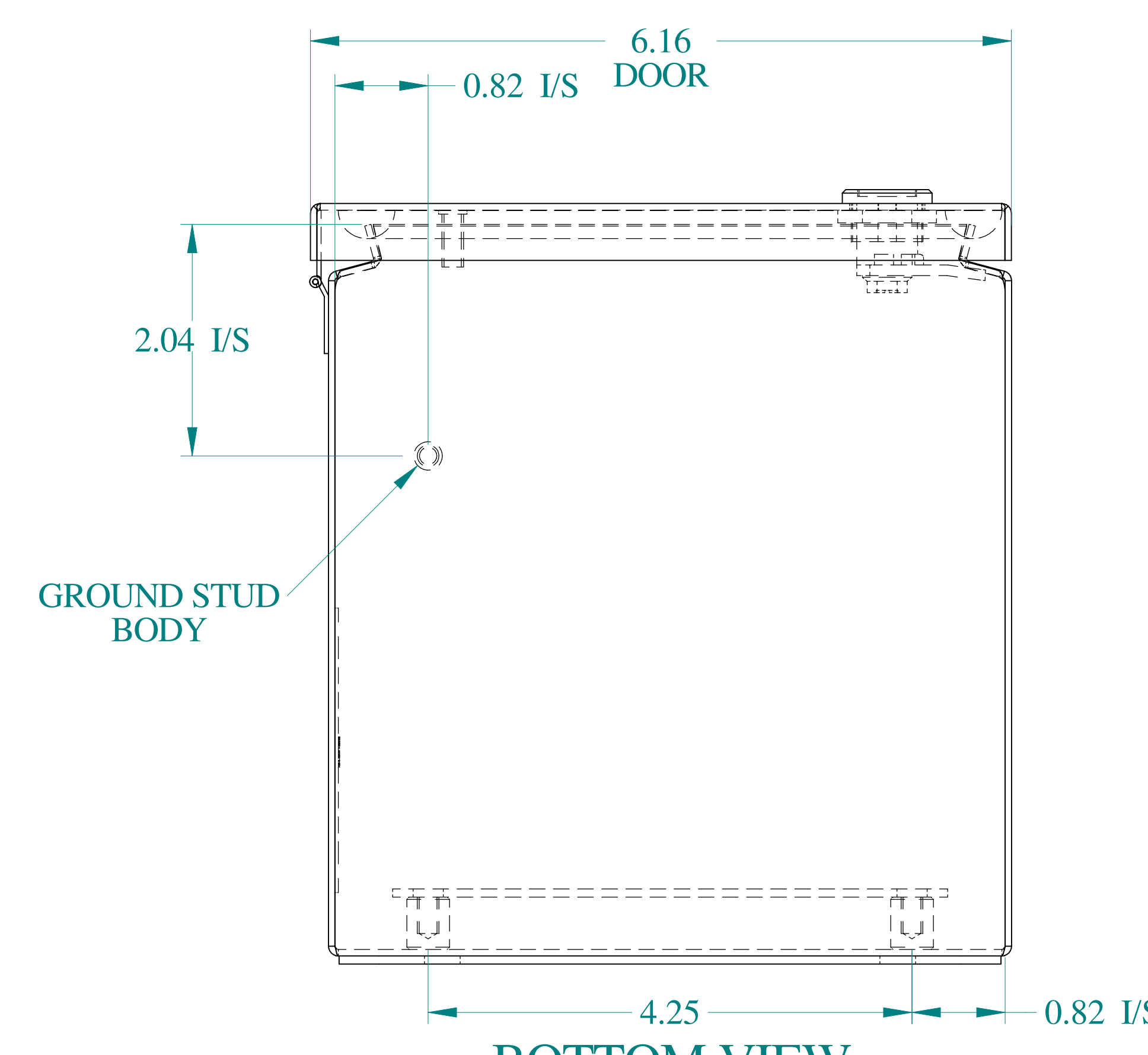
BOTTOM VIEW
