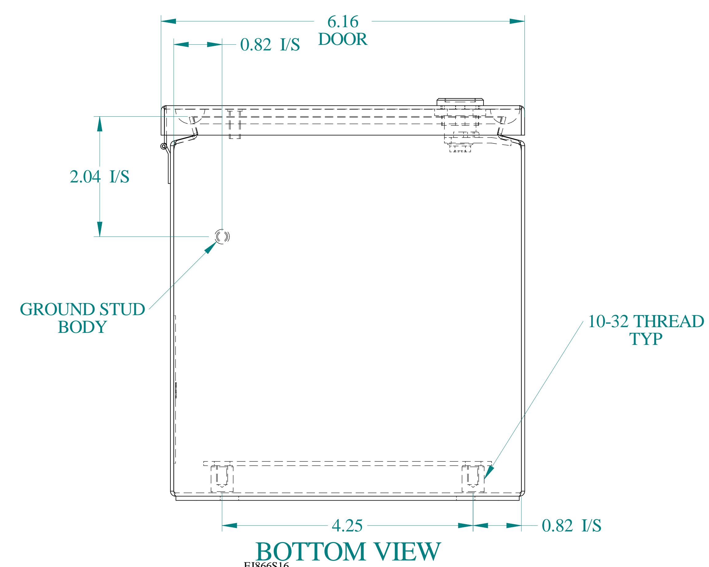
BOTTOM VIEW
