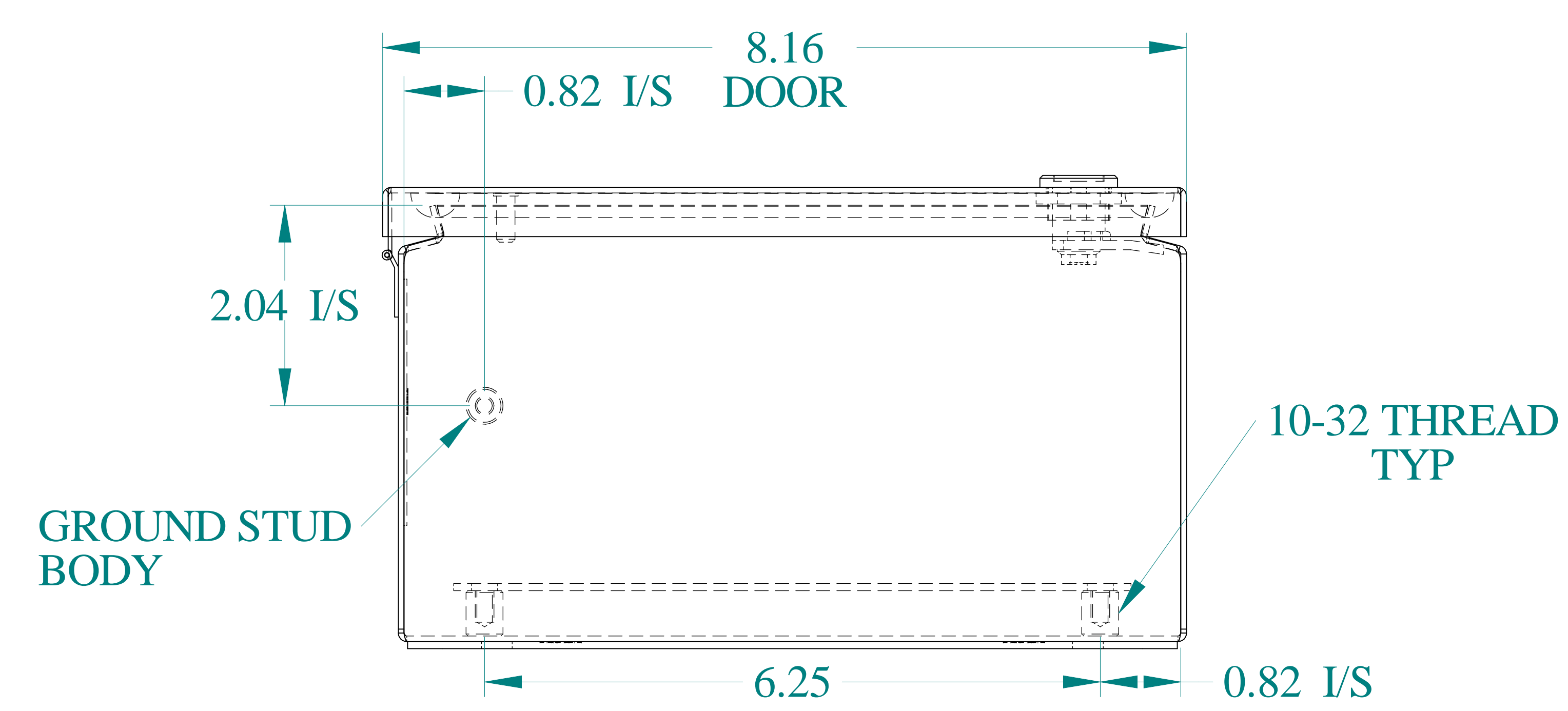
BOTTOM VIEW
