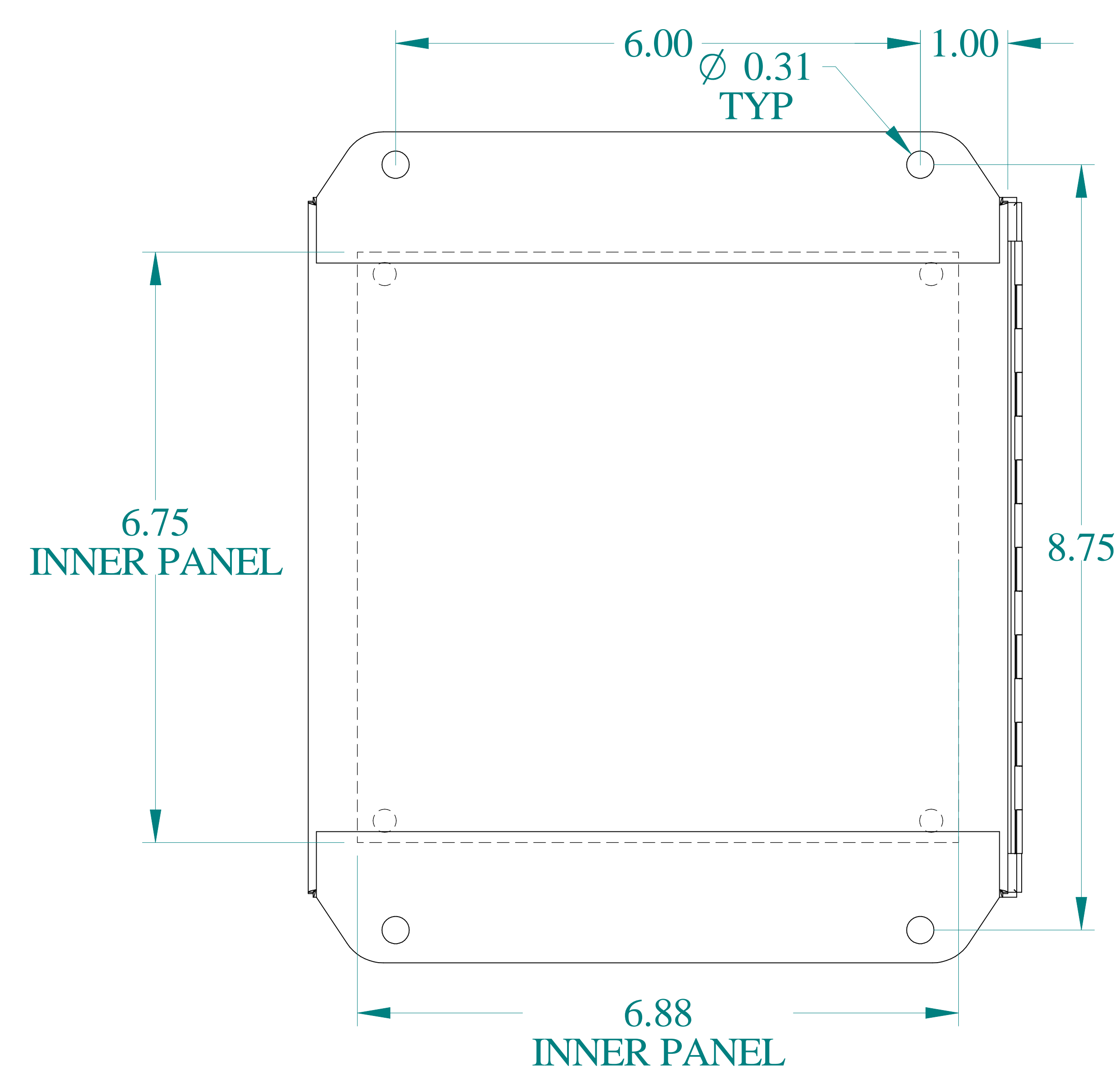
BACK VIEW
