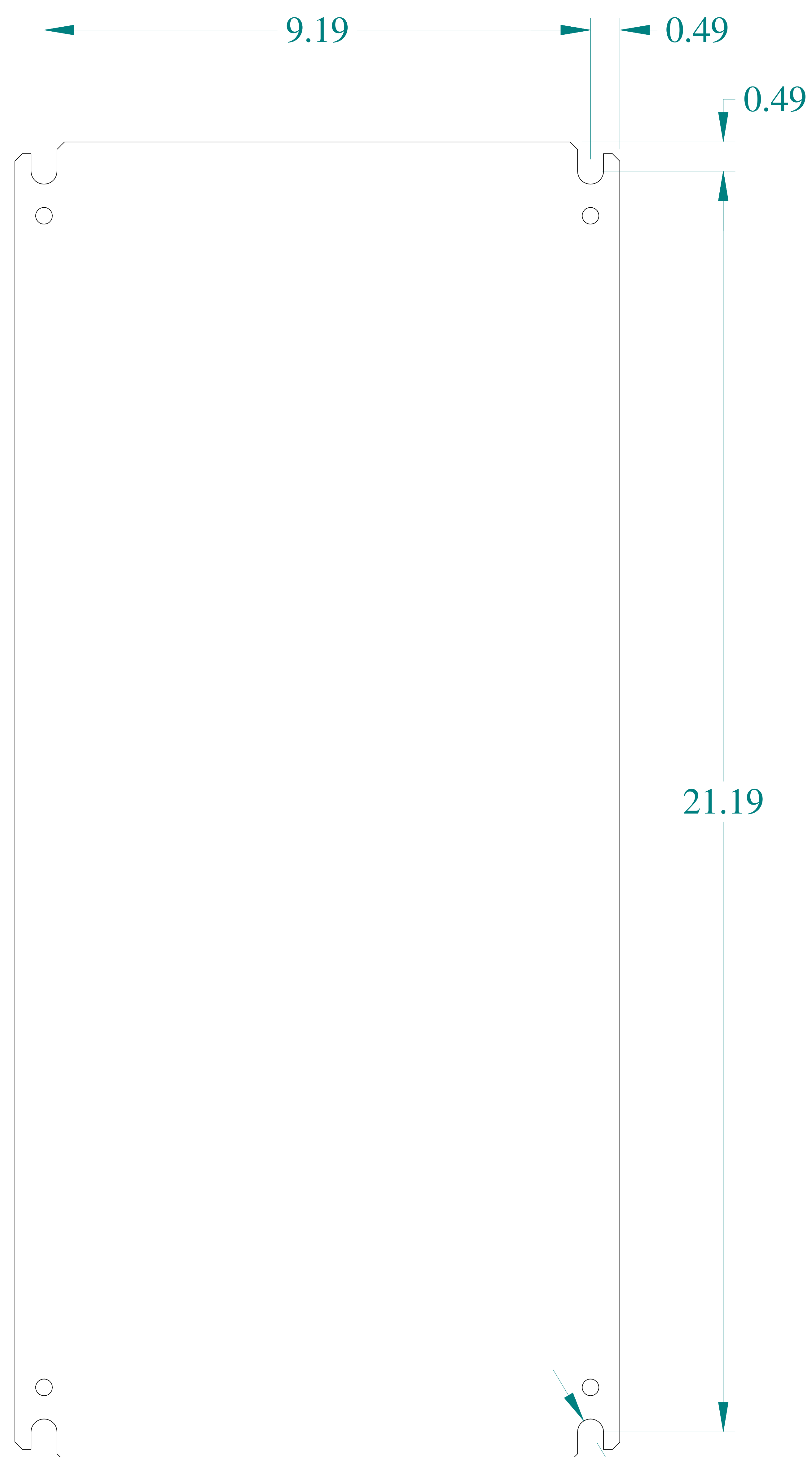
FRONT VIEW
