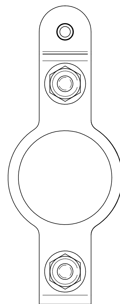
BOTTOM VIEW
